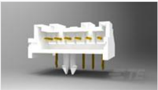
TE Part #1744446-6 Hdr Assy, EP 2.5 RA, 6 Pos., GW
