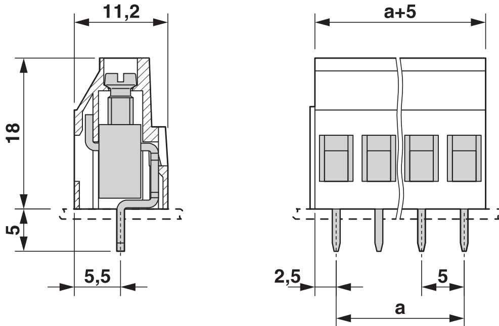
Dimensional drawing
