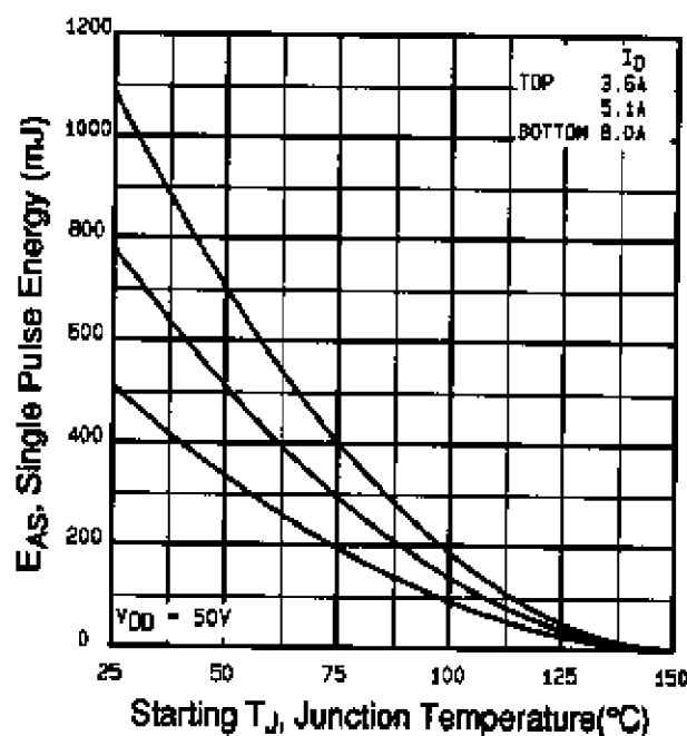
Fig 12c. Maximum Avalanche Energy Vs. Drain Current
