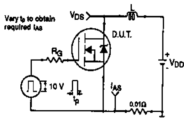
Fig 12a. Unclamped Inductive Test Circuit
