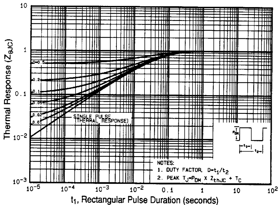
Fig 11. Maximum Effective Transient Thermal Impedance, Junction-to-Case
