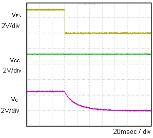
Fig.8 OFF sequence 2 C_o=1.0\mu F
