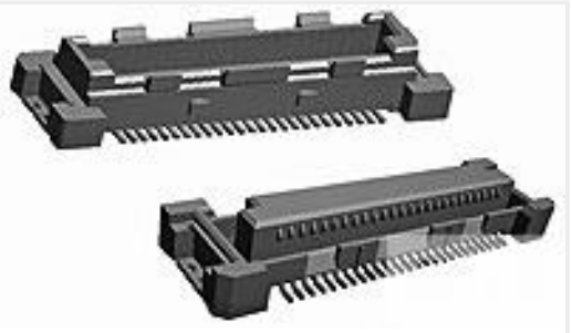
TE Part # 1-5316562-0 .6FHP08H,140,S,GIG,08/Sn,ST,NSYes
