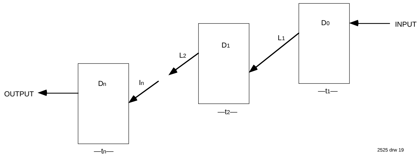
Figure 10. Propagation Delay = t 1 + t 2 + . . . + t n N-Cascaded Devices
