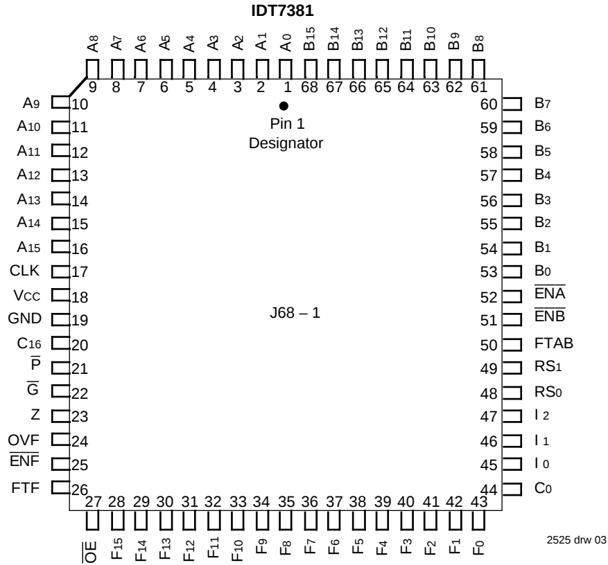
PLCC TOP VIEW
