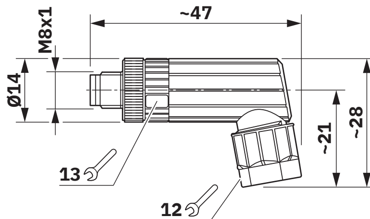
Dimensional drawing
