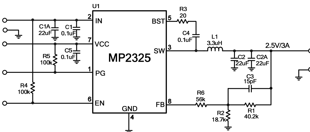
Figure 10: V_o=2.5V , I_o=3A
