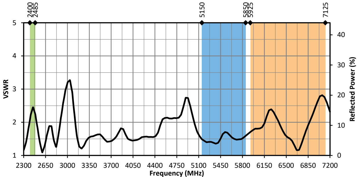
Figure 4. ANT-W63-IPW2-NP VSWR, Free Space
