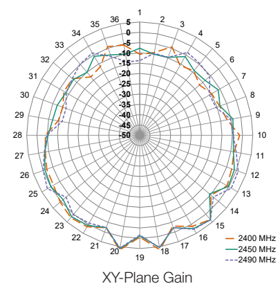
XY-Plane Gain
