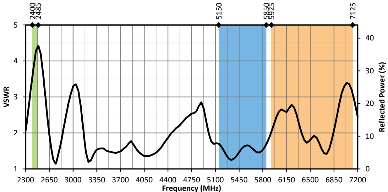
Figure 11. ANT-W63-IPW2-NP Antenna VSWR, Center of Ground Plane
