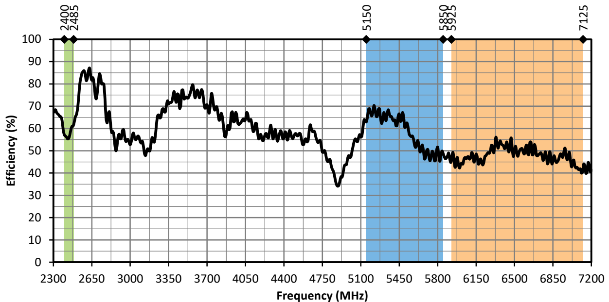
Figure 8. ANT-W63-IPW2-NP Series Antenna Radiation Efficiency, Free Space
