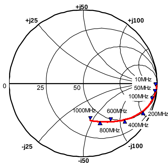
S_{22} (Circuit 5, \text{Pin}= -10\text{dBm} )
