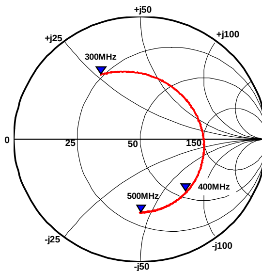
RF OUT Output Impedance Z_{out} (Circuit 3, \text{Pin}=0\text{dBm} )
