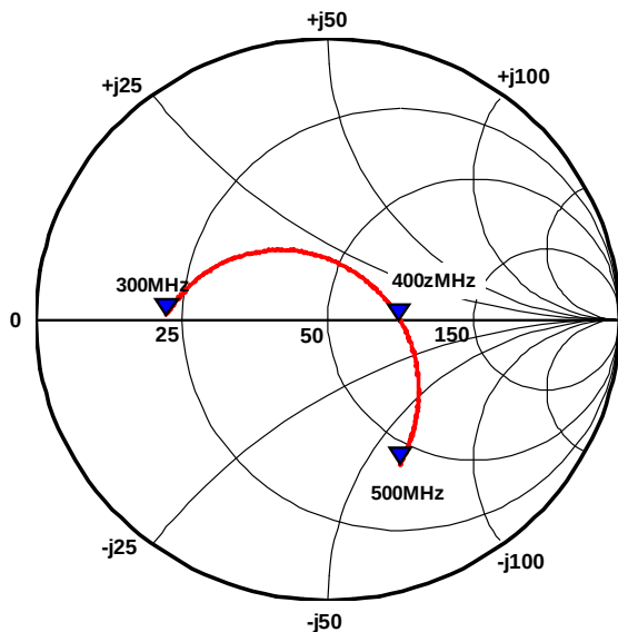
RF IN Input Impedance Z_{in} (Circuit 3, \text{Pin}=0\text{dBm} )
