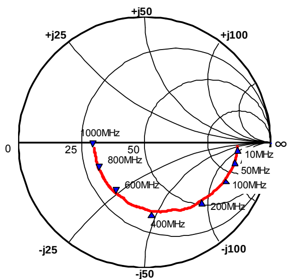
S_{11} (Circuit 5, \text{Pin}= -10\text{dBm} )
