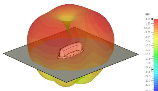
650 MHz, side view
