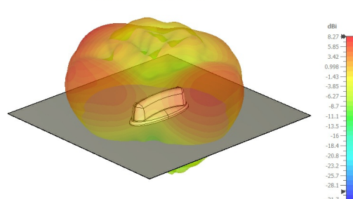
2100 MHz, side view
