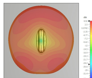
800 MHz, top view
