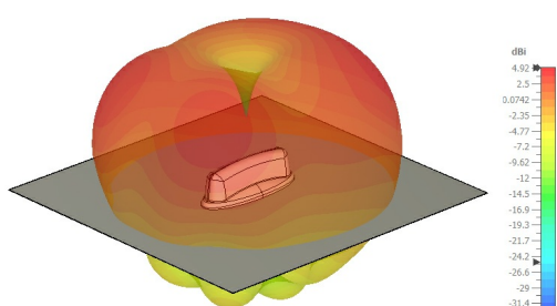
800 MHz, side view
