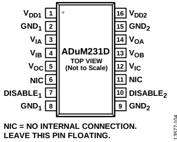
Figure 8. ADuM231D Pin Configuration
