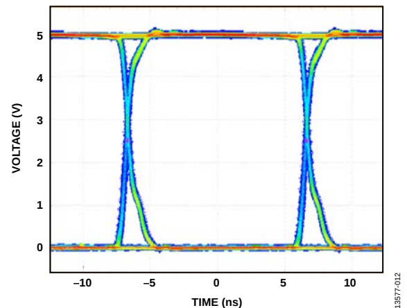
Figure 20. Eye Diagram
