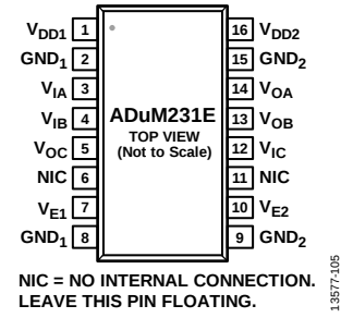
Figure 9. ADuM231E Pin Configuration
