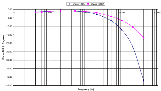
CP1005 Phase Response
