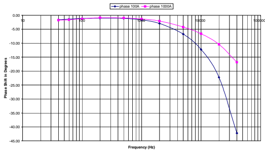
CP1005 Phase Response
