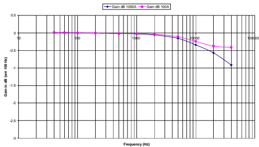
CP1005 Frequency Response
