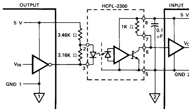
Figure 14. Series Drive from Open Collector TTL/LSTTL Units.
