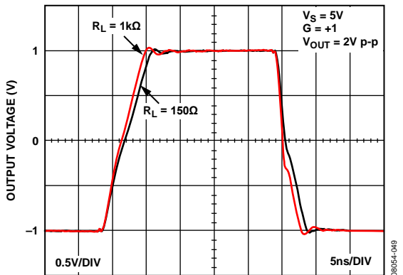
Figure 33. Large-Signal Step Response, V_S = 5\text{ V} , G = +1
