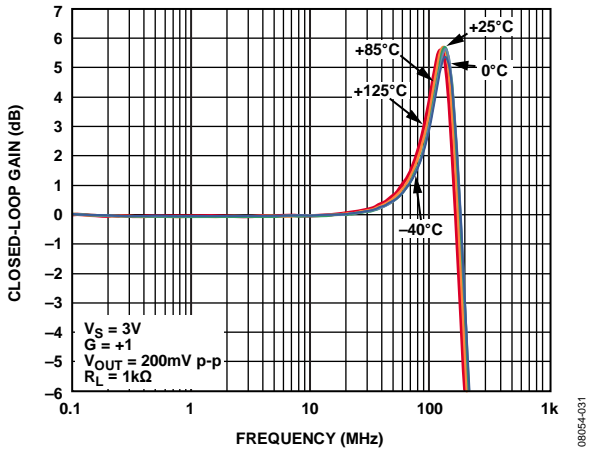
Figure 13. Small-Signal Frequency Response vs. Temperature, V_S = 3V , ADA4891-1/ADA4891-2
