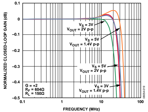
Figure 14. 0.1 dB Gain Flatness vs. Supply Voltage, G = +2 , ADA4891-1/ADA4891-2
