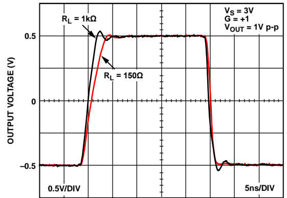
Figure 36. Large-Signal Step Response, V_S = 3\text{ V} , G = +1
