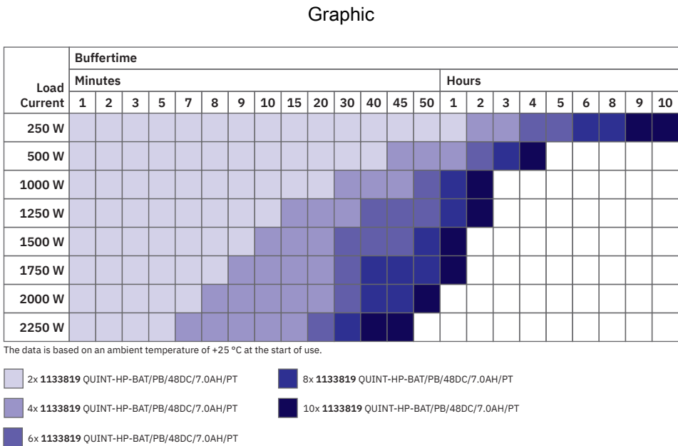
QUINT HP UPS 2.5 kVA buffer times
