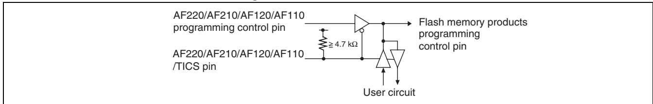
Figure 28.2-2 Control Circuit
