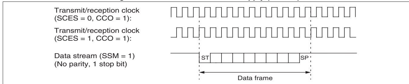
Figure 22.7-6 Continuous Clock Supply (Mode 2)
