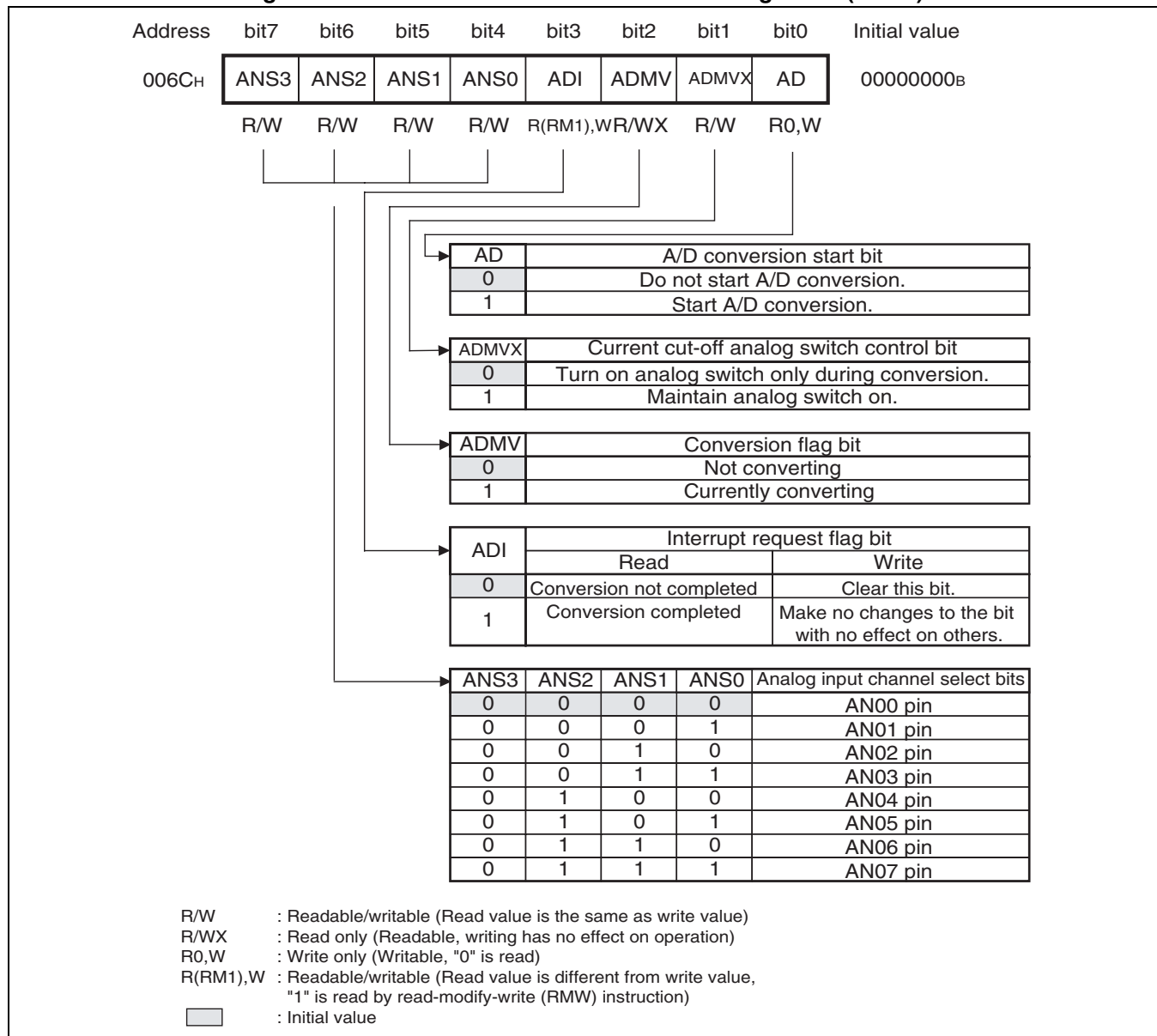
Figure 24.4-2 8/10-bit A/D Converter Control Register 1 (ADC1)
