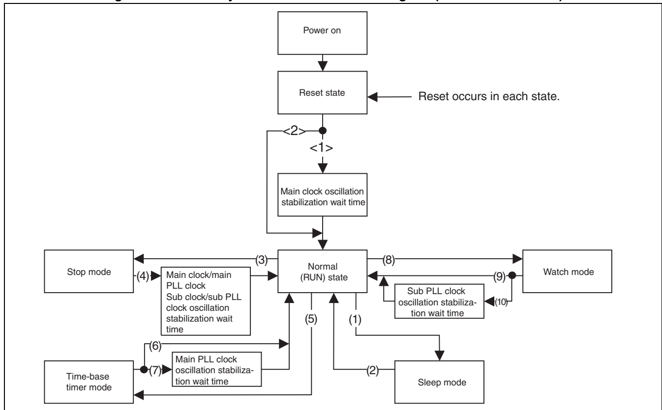
Figure 6.8-1 Standby Mode State Transition Diagram (Dual Clock Product)
