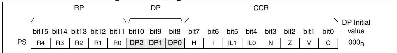
Figure 5.1-4 Configuration of Direct Bank Pointer
