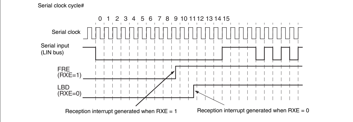
Figure 22.7-8 LIN-UART Operation in LIN Slave Modes
