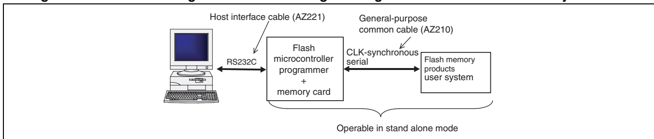
Figure 28.1-1 Basic Configuration of Serial Programming Connection for Flash Memory Products
