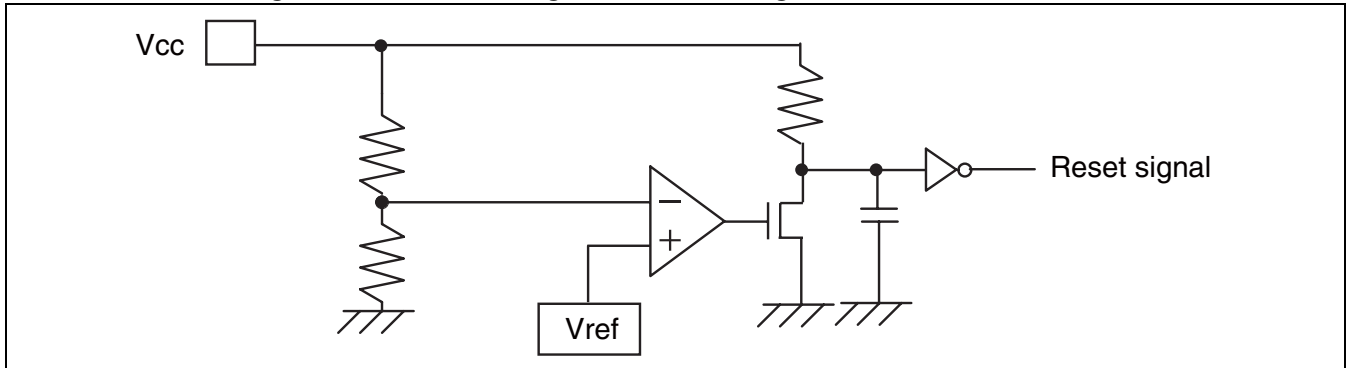
Figure 25.2-1 Block Diagram of Low-voltage Detection Reset Circuit
