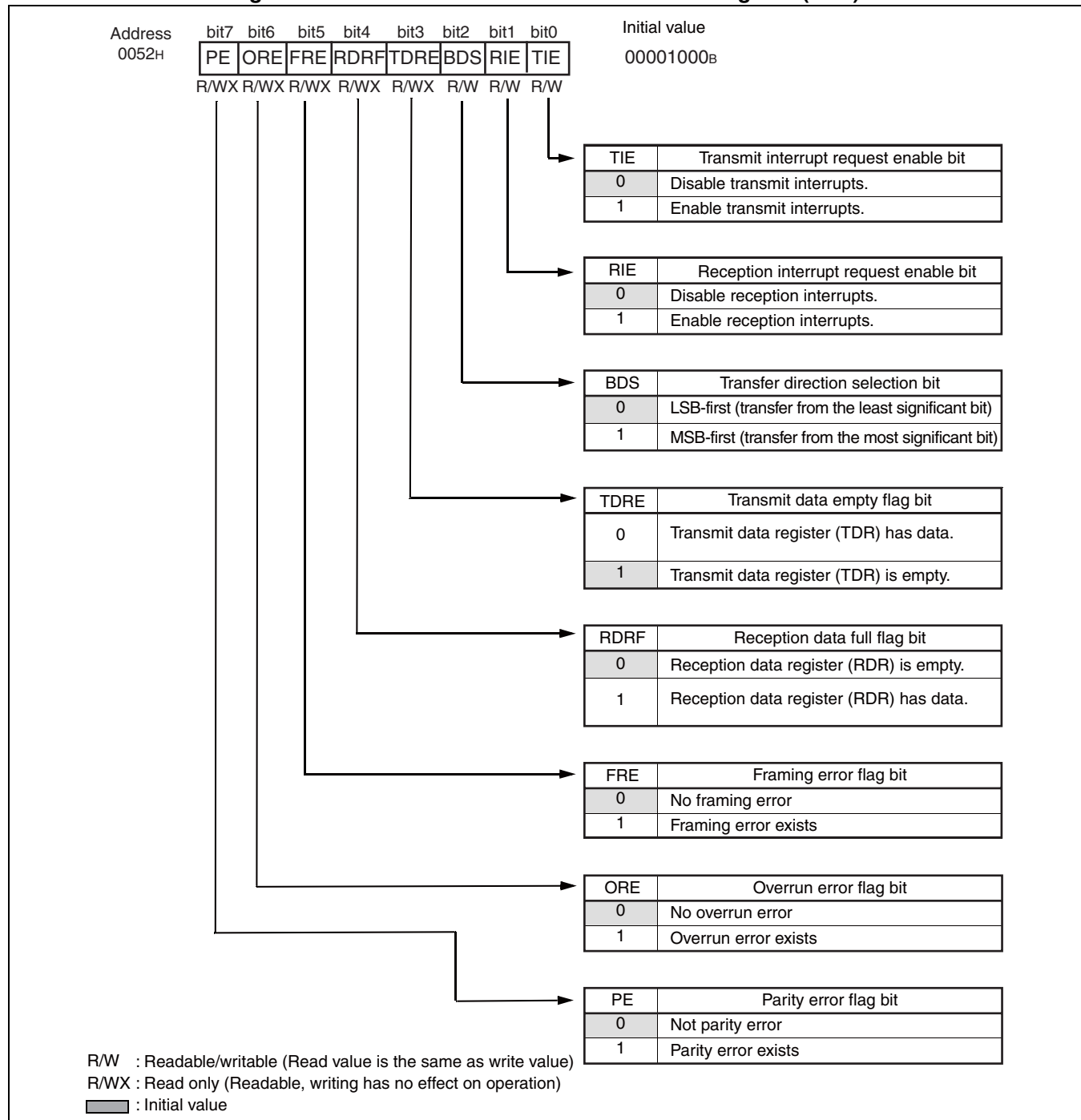
Figure 22.4-4 LIN-UART Serial Status and Data Register (SSR)
