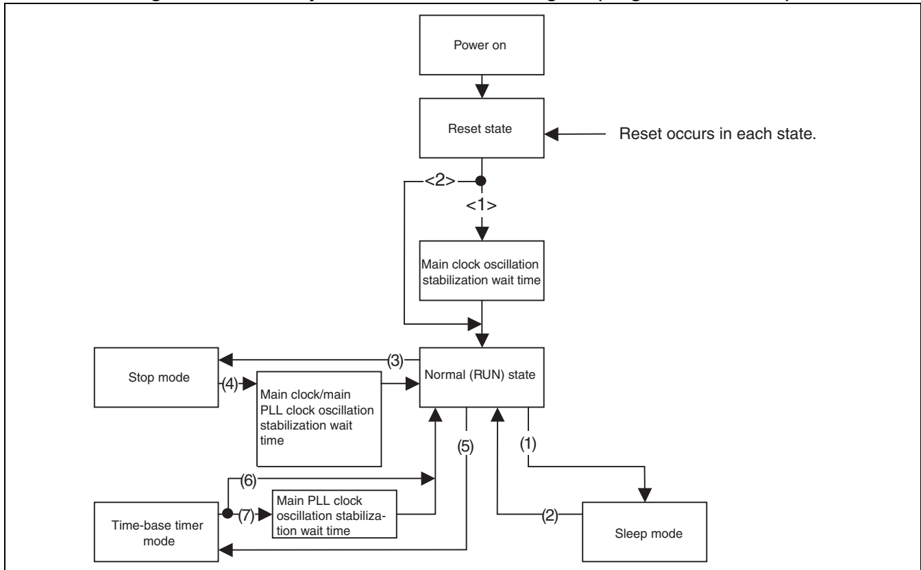
Figure 6.8-2 Standby Mode State Transition Diagram (Single Clock Product)
