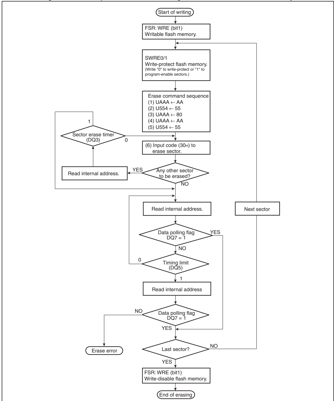
Figure 27.6-2 Sample Procedure for Erasing Data from Sectors in Flash Memory
