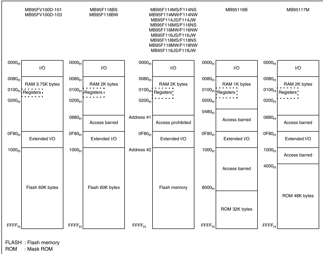
Figure C-1 Memory Map
