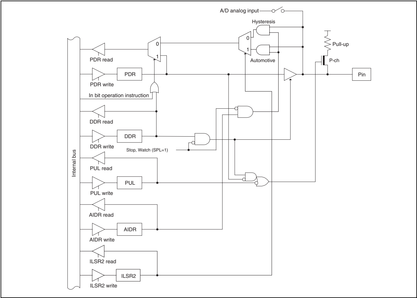
Figure 24.3-1 Block Diagram of Pins (AN00 to AN07) Related to 8/10-bit A/D Converter
