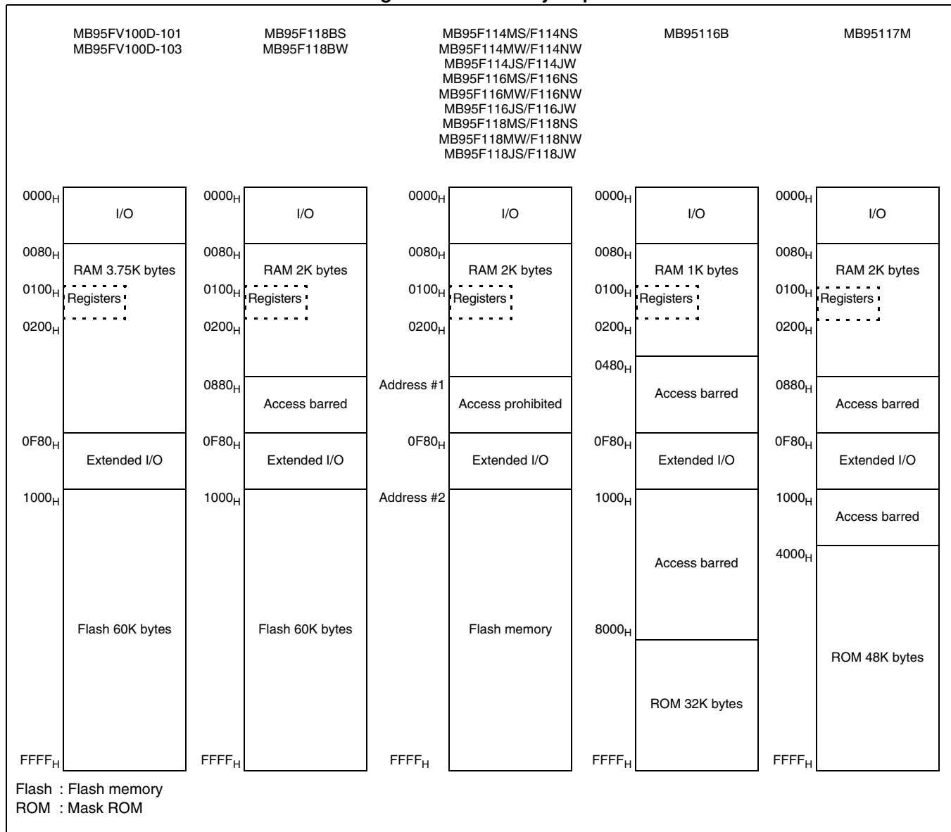
Figure 3.2-1 Memory Map
