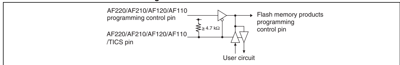
Figure 28.1-2 Control Circuit
