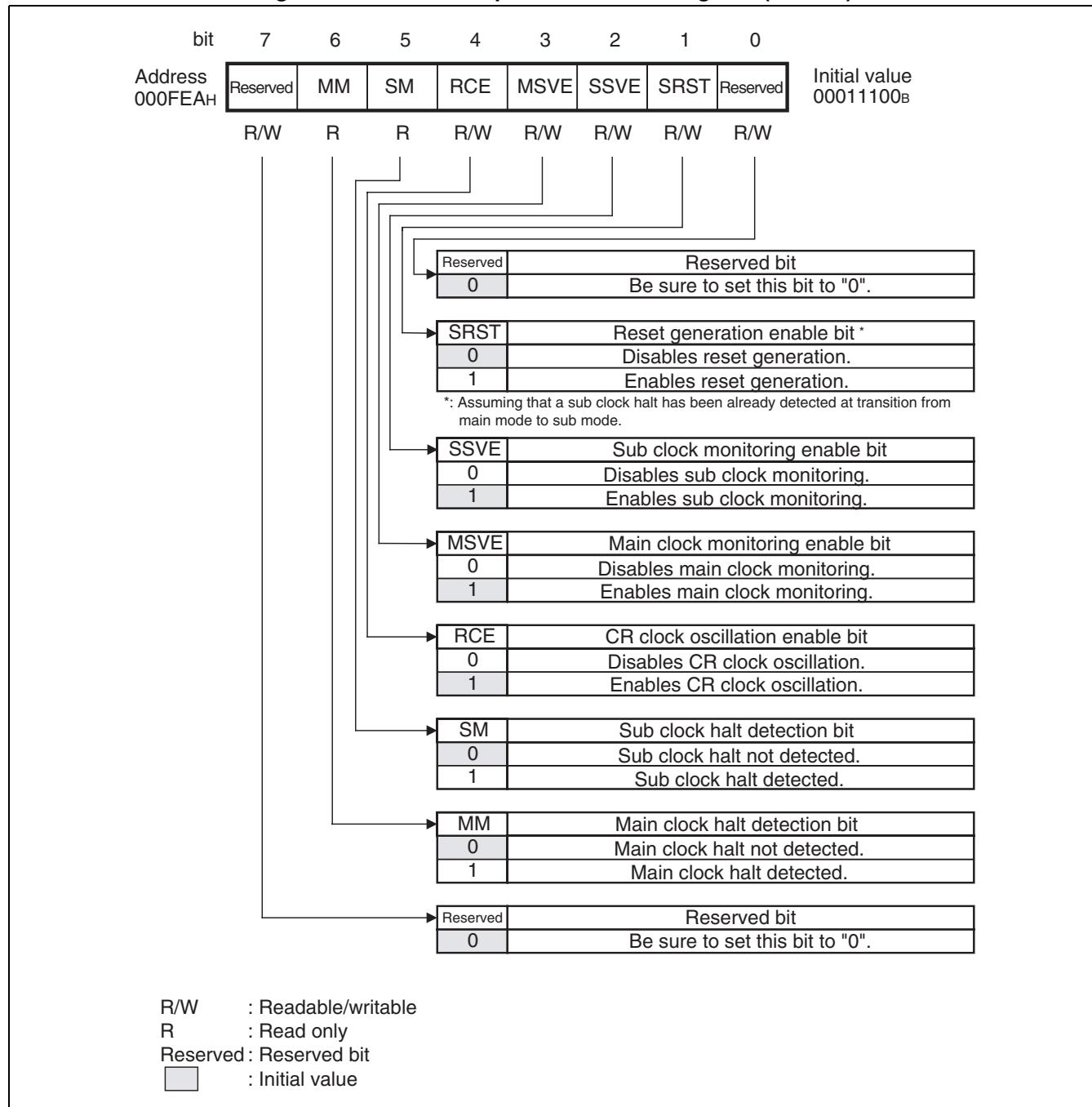
Figure 26.3-2 Clock Supervisor Control Register (CSVCR)
