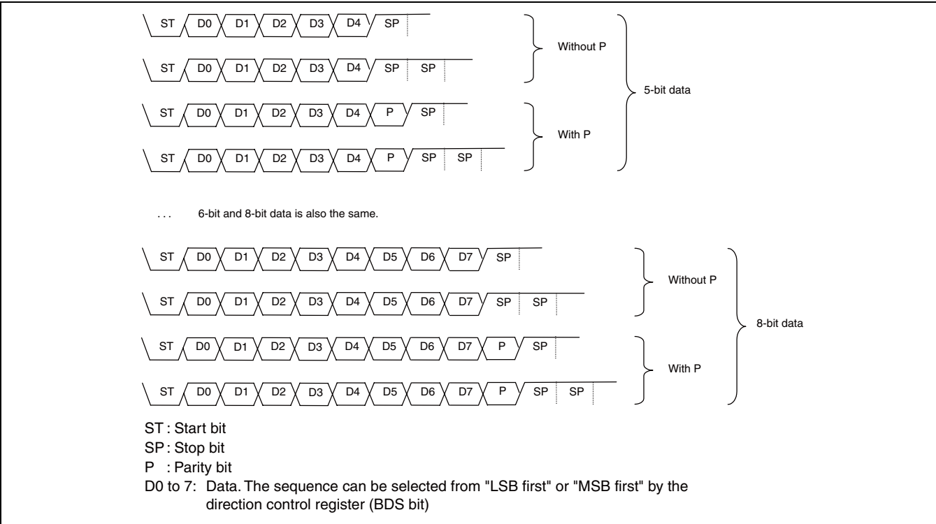
Figure 20.7-2 Transfer Data Format
