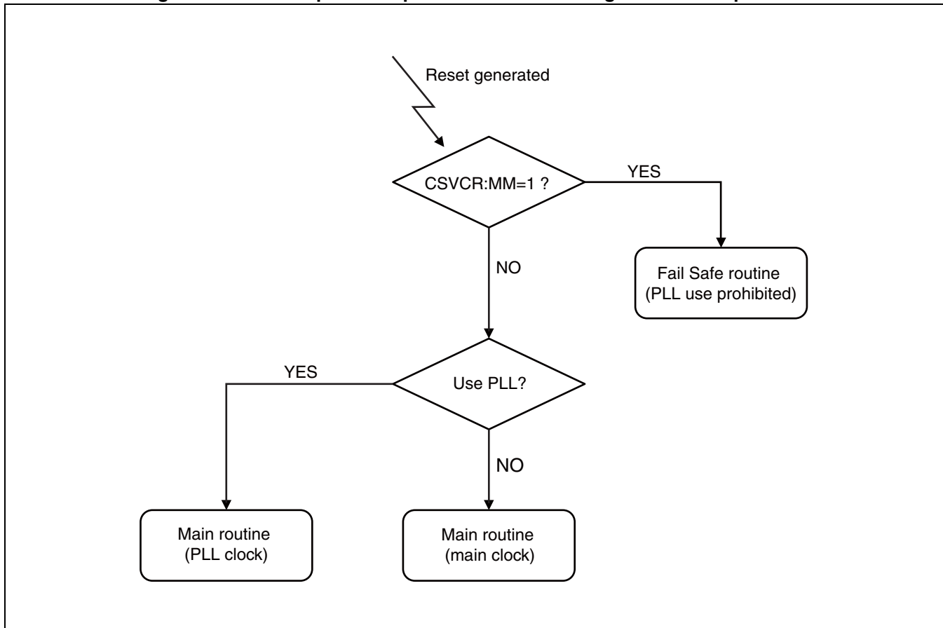
Figure 26.4-2 Example Startup Flowchart when using the Clock Supervisor
