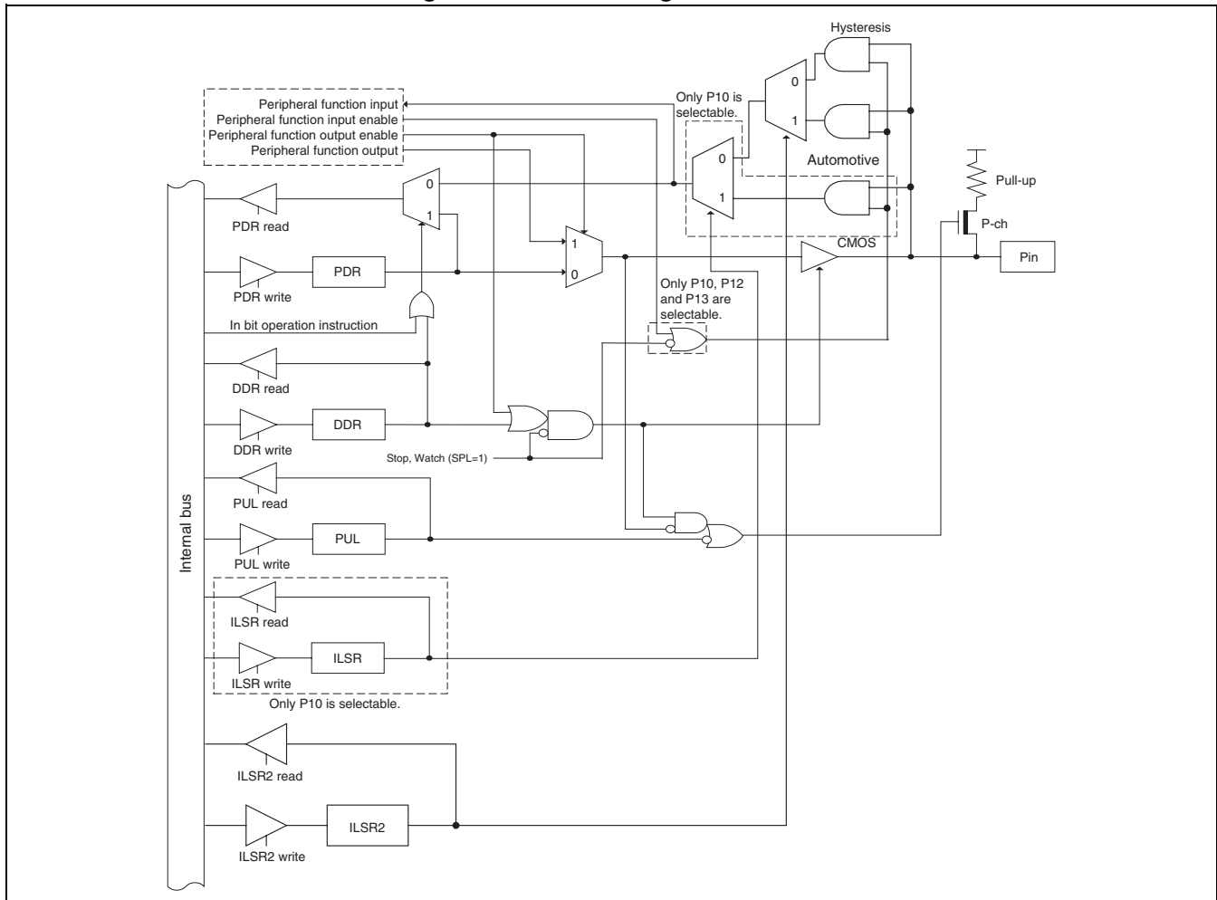
Figure 9.3-1 Block Diagram of Port 1
