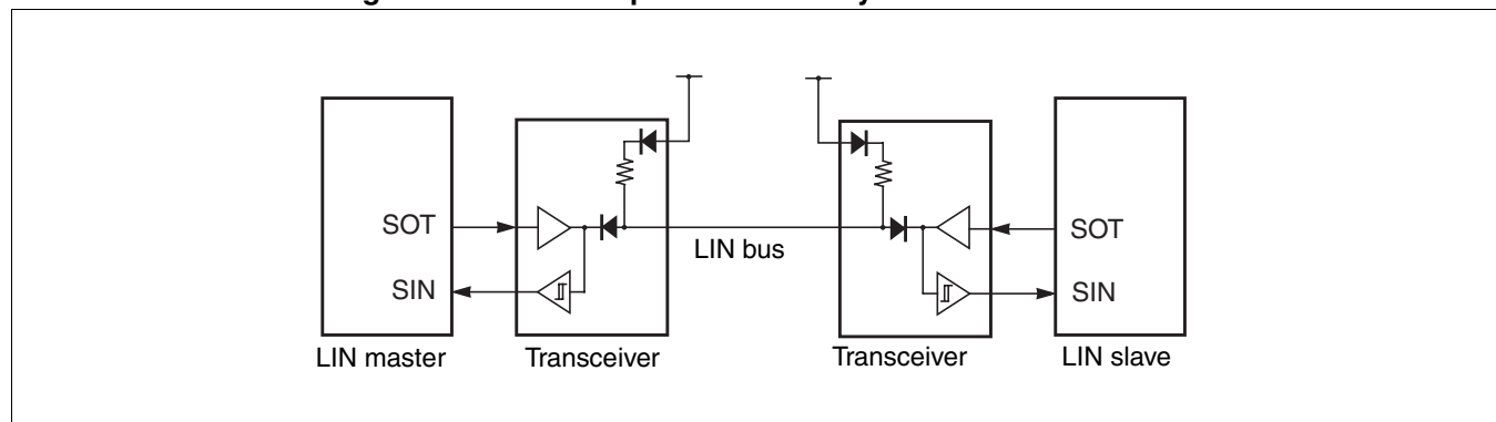
Figure 22.7-17 Example of LIN Bus System Communication
