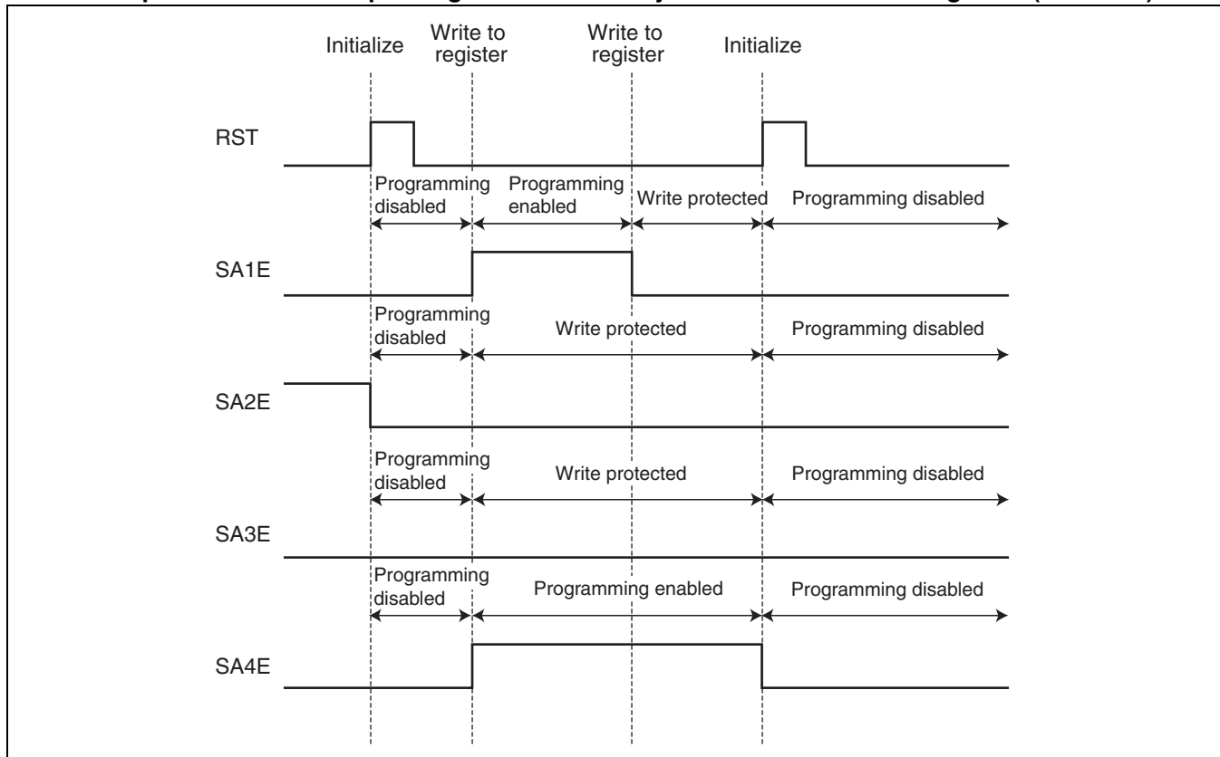
Figure 27.3-4 Examples of Flash Memory Programming-disabled, Programming-enabled, and Write-protected States Depending on Flash Memory Sector Write Control Registers (SWRE0/1)
