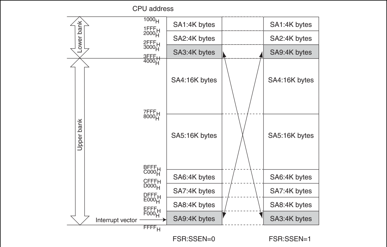
Figure 29.2-1 Access Sector Map by FSR:SSEN Value
