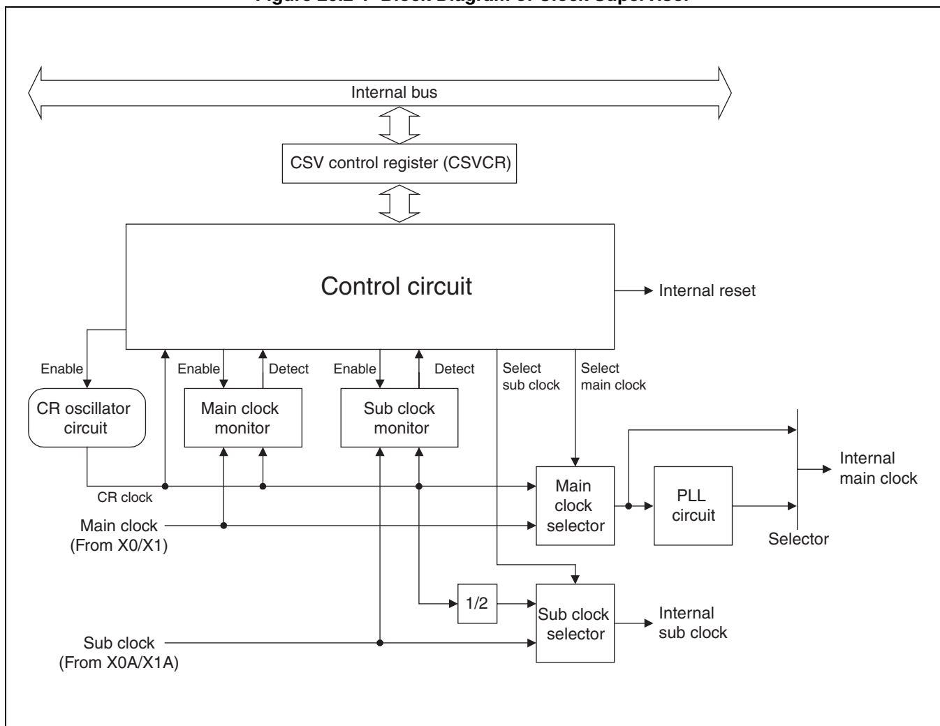
Figure 26.2-1 Block Diagram of Clock Supervisor
