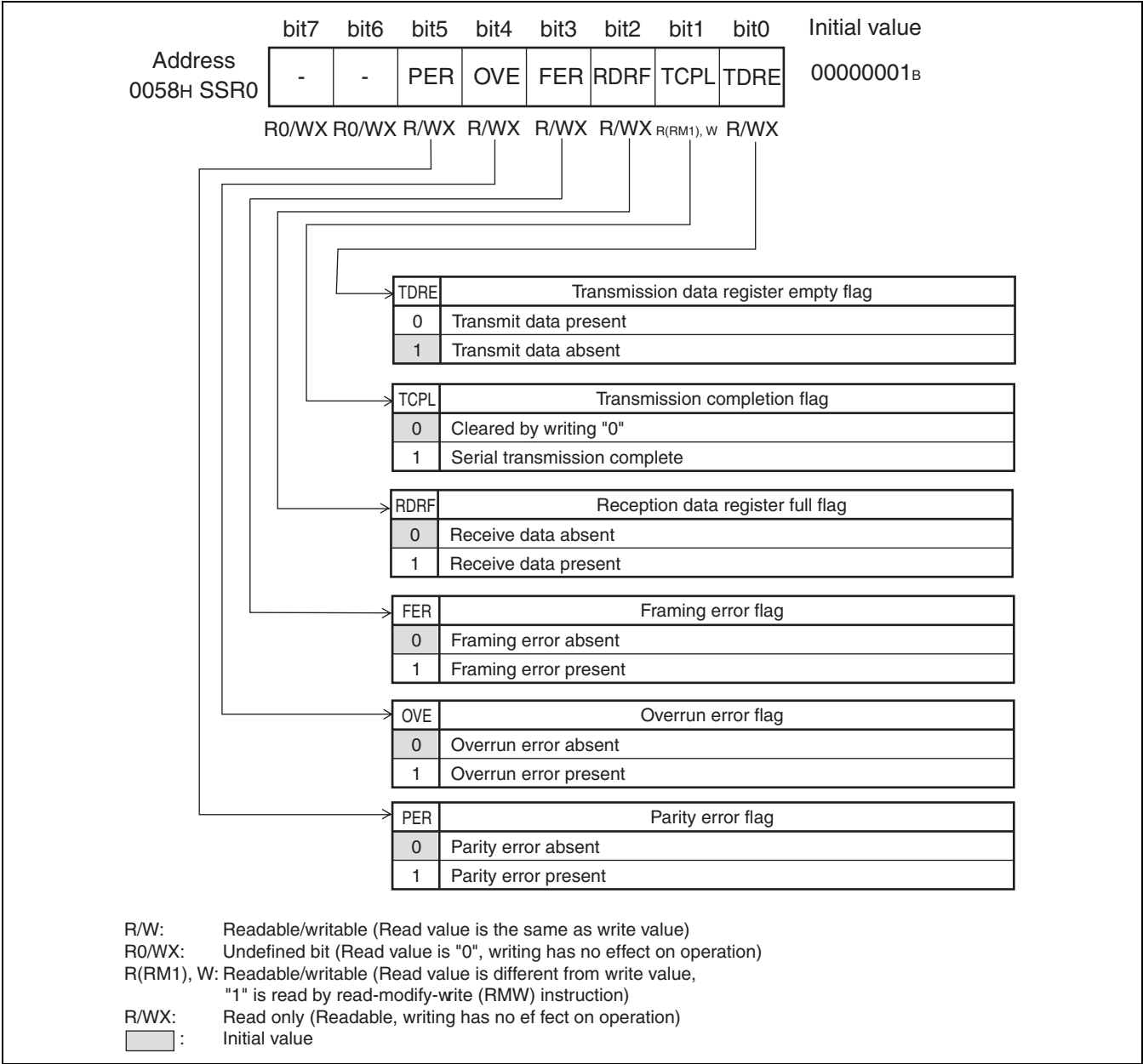
Figure 20.5-4 UART/SIO Serial Status and Data Register (SSR0)
