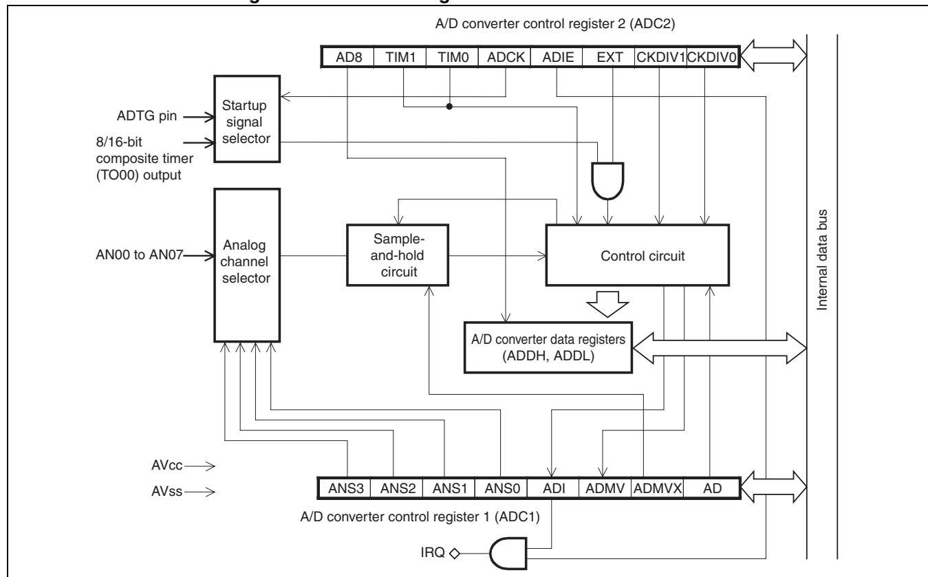
Figure 24.2-1 Block Diagram of 8/10-bit A/D Converter
