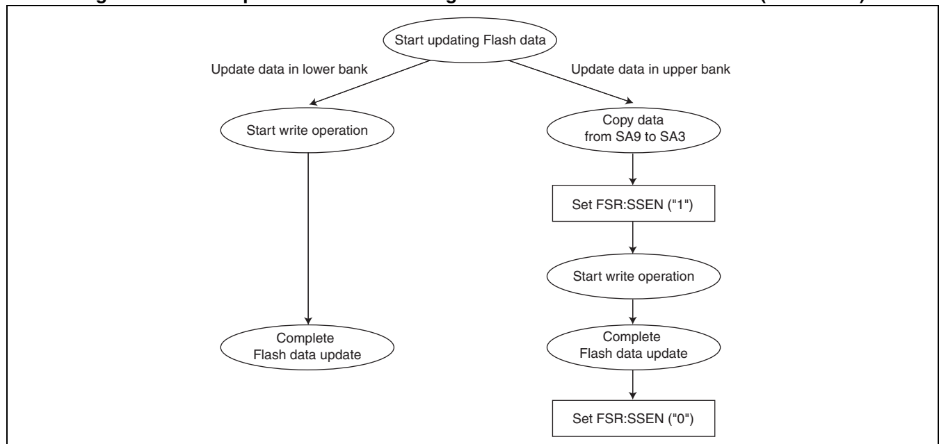
Figure 29.3-1 Sample Procedure of Setting the Sector Conversion Enable Bit (FSR:SSEN)
