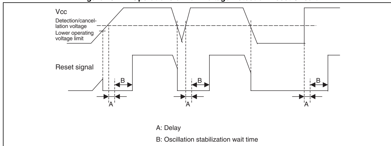
Figure 25.4-1 Operations of Low-voltage Detection Reset Circuit
