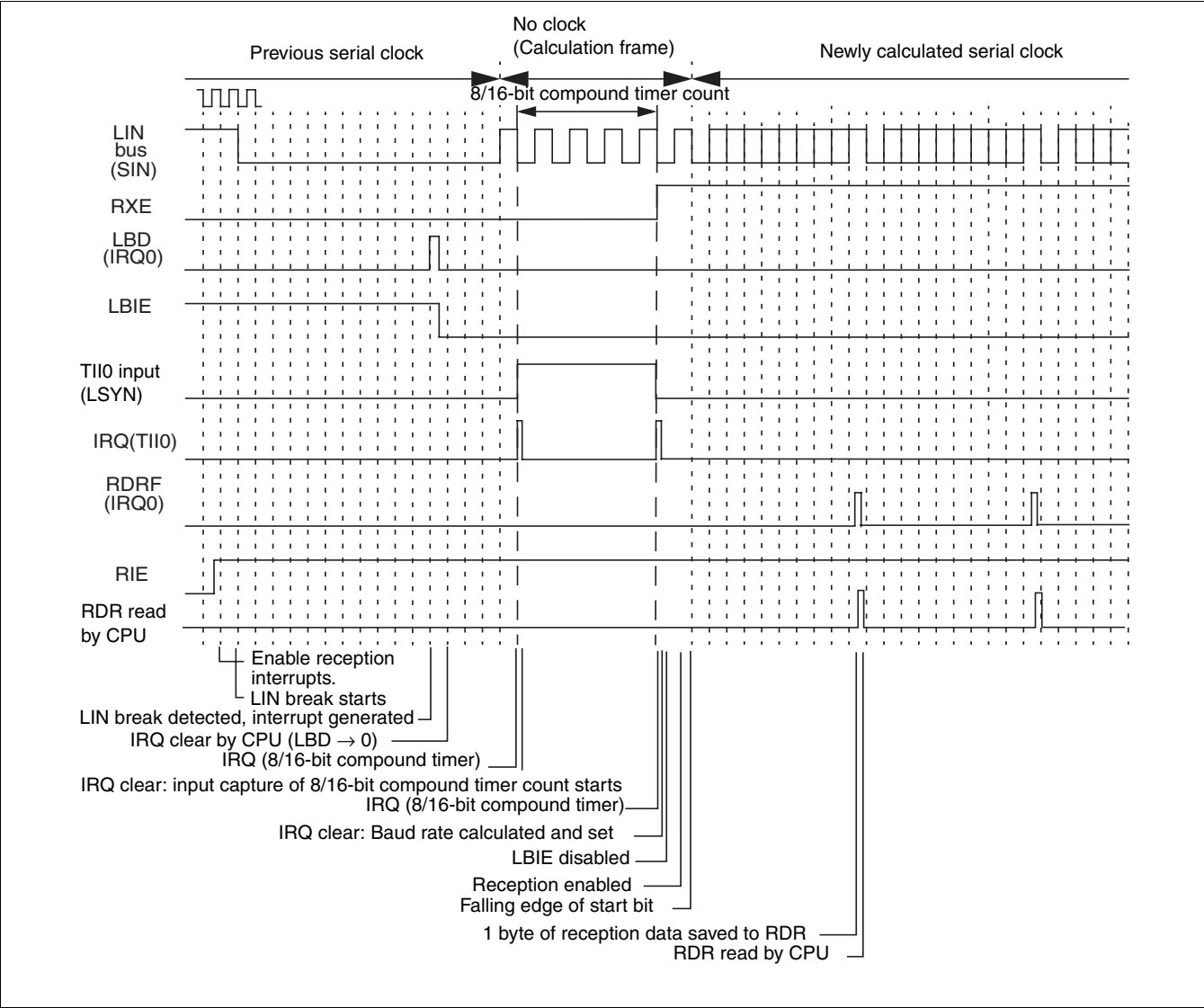
Figure 22.7-9 LIN Bus Timing and LIN-UART Signals
