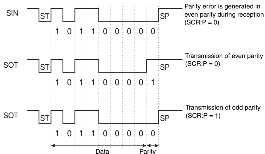
Figure 22.7-2 Transmission Data when Parity is Enabled
