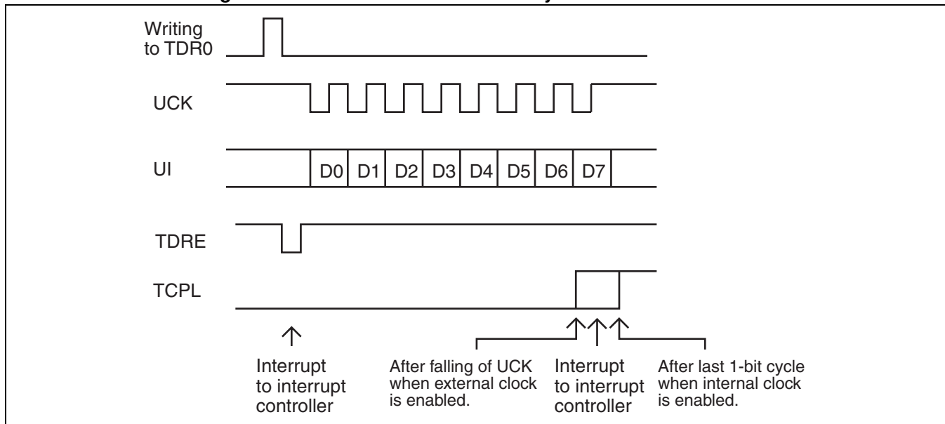
Figure 20.7-14 8-bit Transmission in Synchronous CLK Mode
