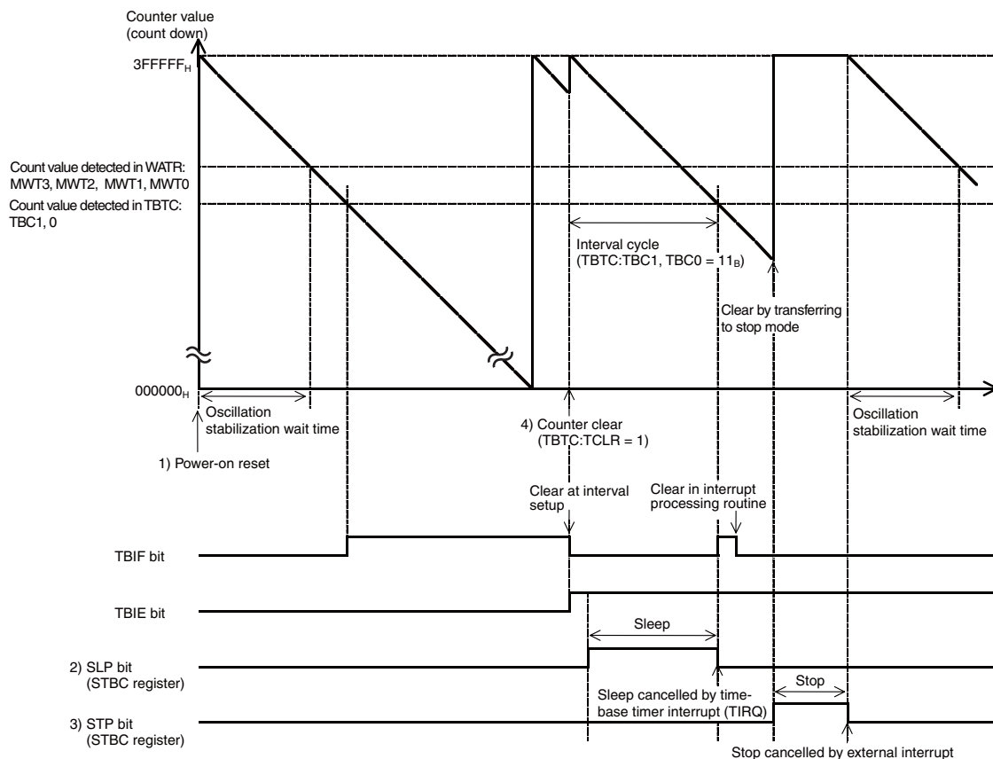
Figure 10.5-2 Operations of Time-base Timer
