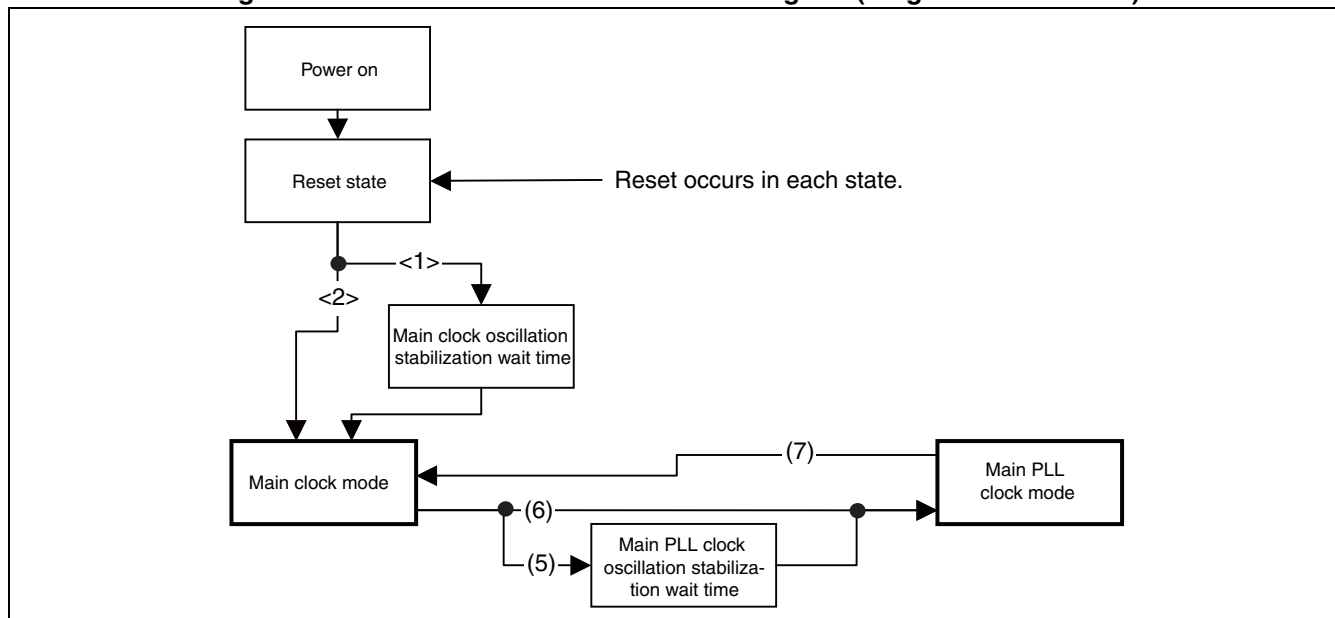
Figure 6.7-2 Clock Mode State Transition Diagram (Single Clock Product)
