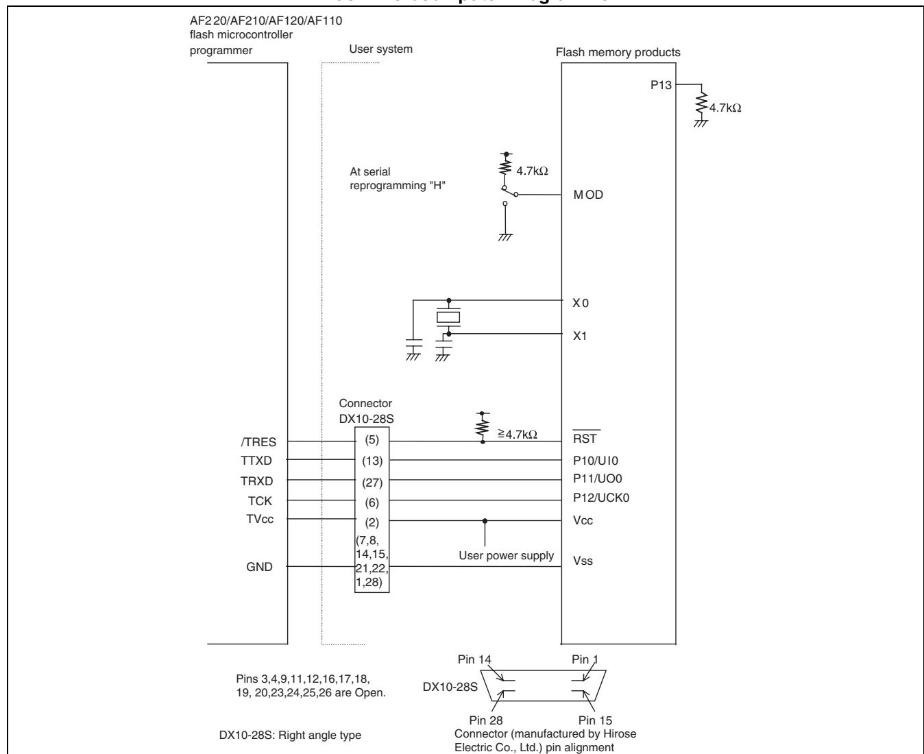
Figure 28.3-1 Example of Minimum Connection between Flash Memory Products and Flash Microcomputer Programmer
