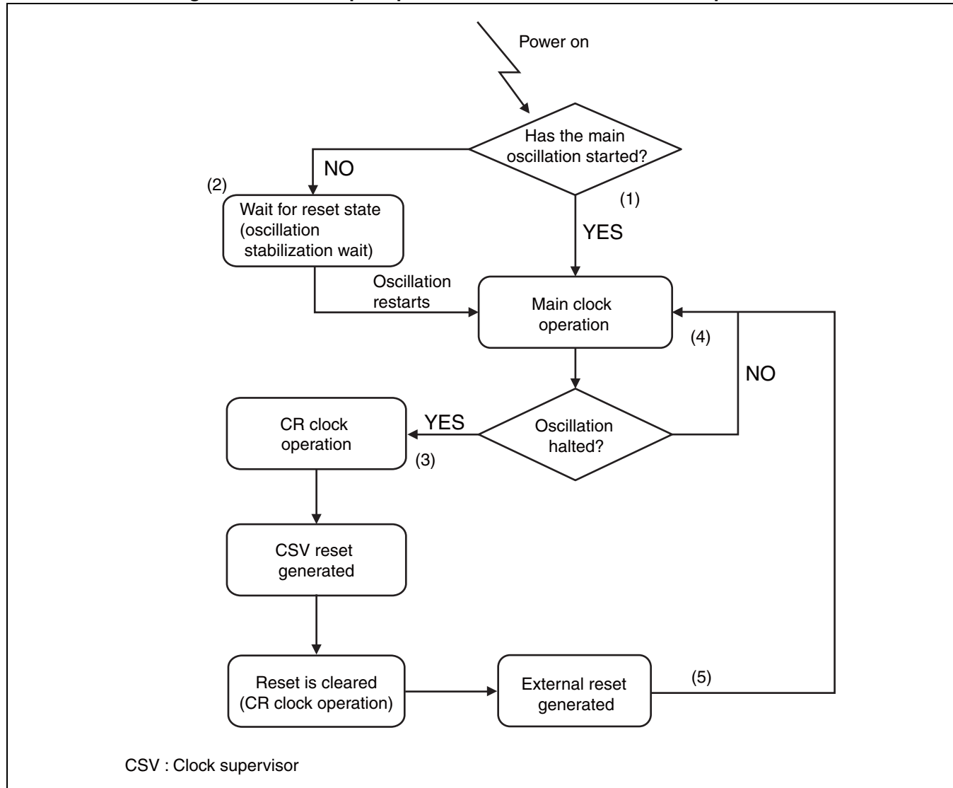
Figure 26.4-1 Example Operation Flowchart for the Clock Supervisor
