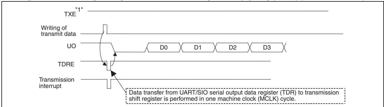
Figure 20.7-7 Setting Timing 1 for Transmit Data Register Empty Flag (TDRE) (When TXE is "1")
