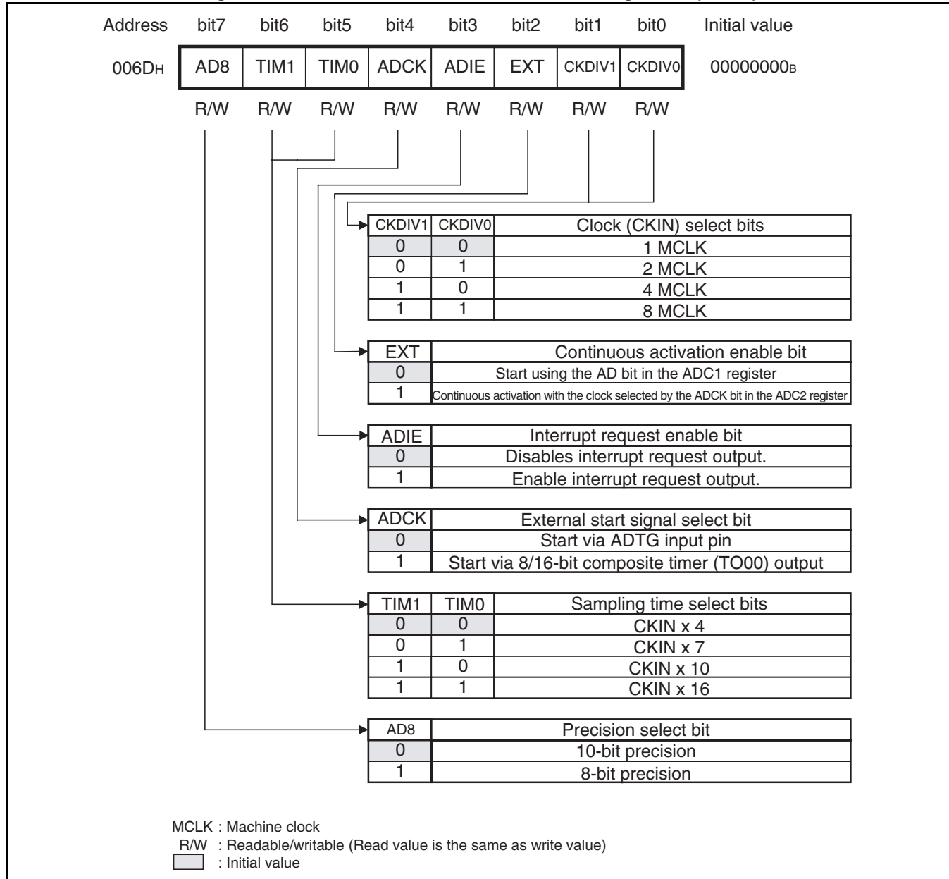
Figure 24.4-3 8/10-bit A/D Converter Control Register 2 (ADC2)
