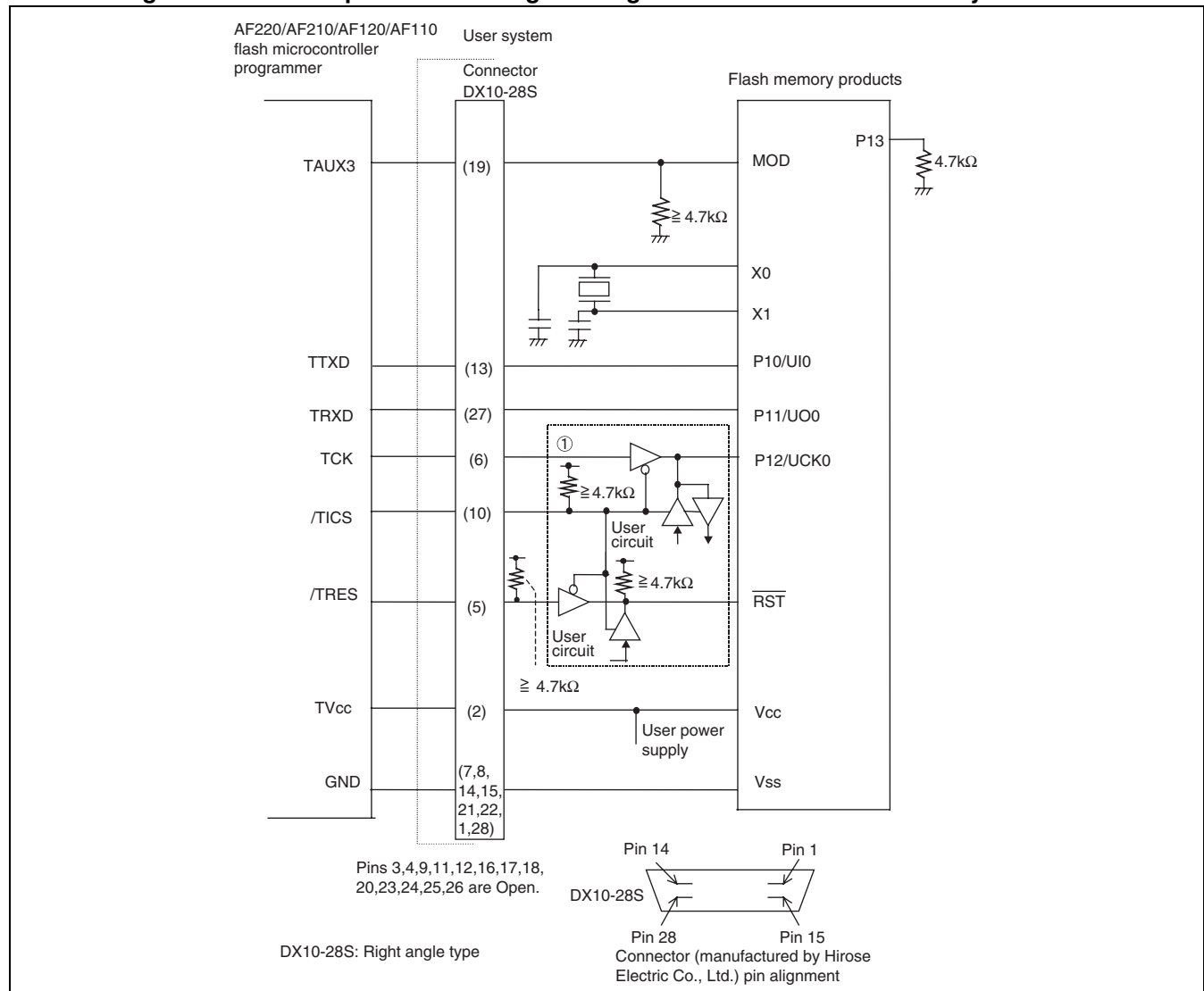
Figure 28.2-1 Example of Serial Programming Connection for Flash Memory Products
