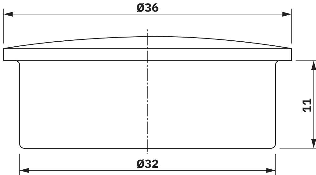
Dimensional drawing
