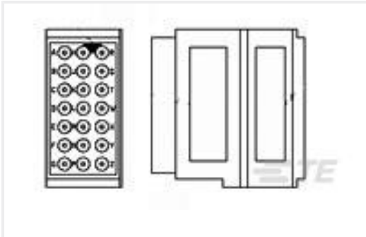
TE Part #592629-7 TERM JCT,F/B SZ 21,34 BUSS
