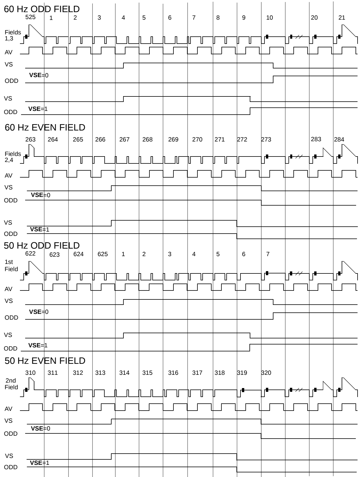
Figure 22. Vertical Timing
