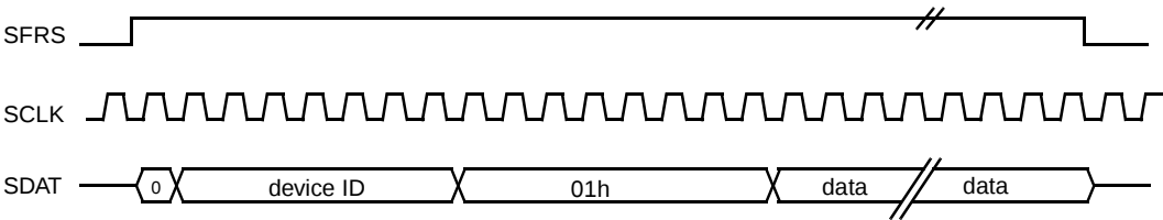
Figure 26. A Typical 3-wire Write to Data Register
