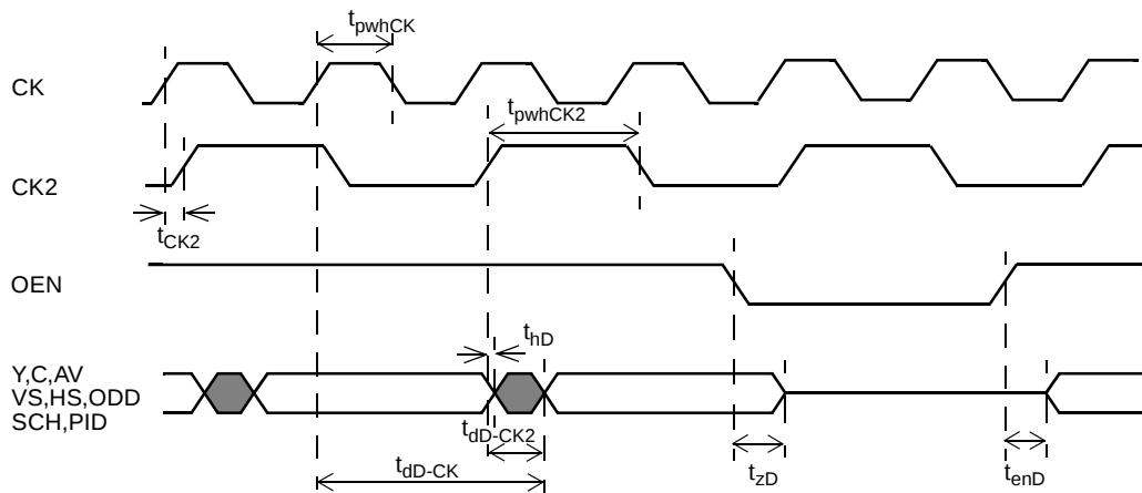
Figure 29. Data Output
