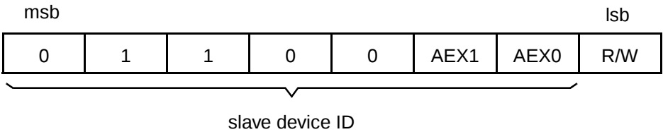
Figure 27. 2-wire Slave Device ID and R/W
