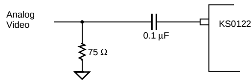
Figure 1. Typical Analog Video Input
