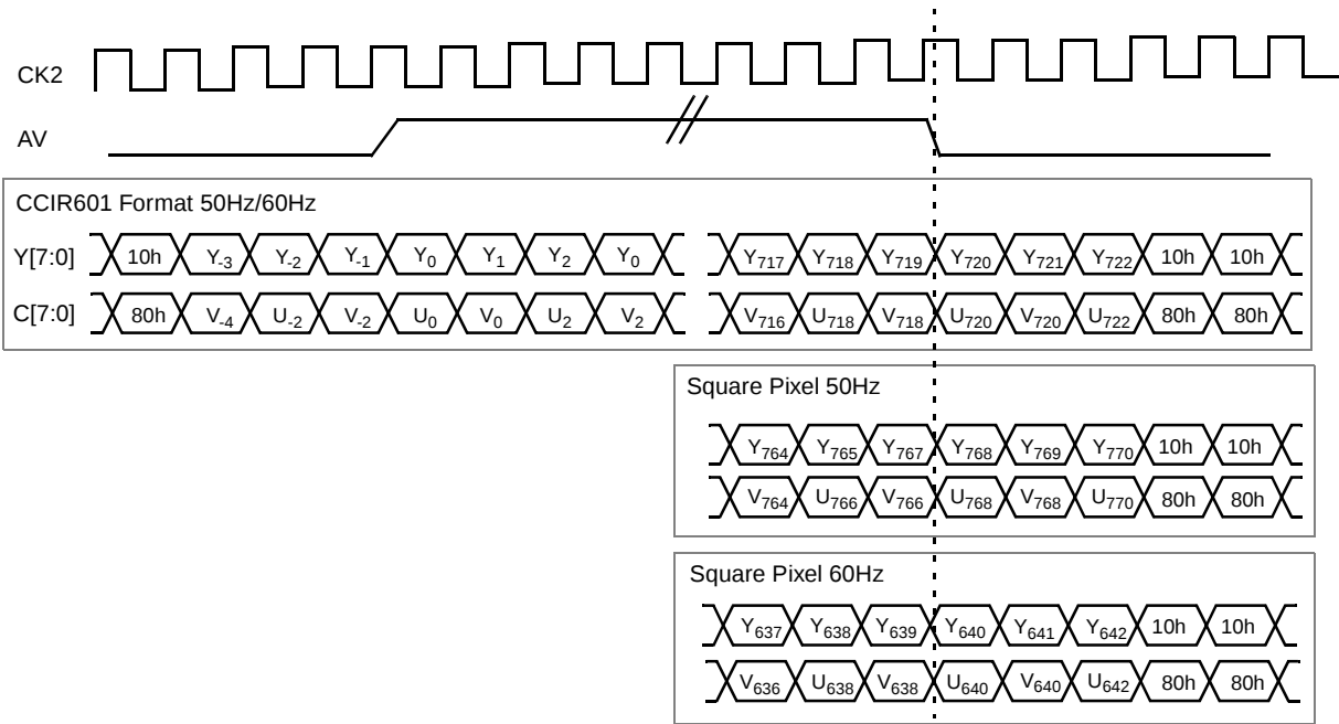
Figure 23. Data Output for 4:2:2 Format
