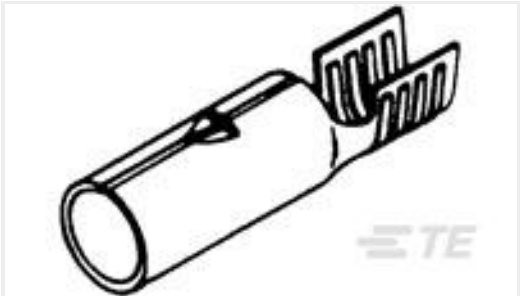
TE Part #42868-2 SHUR PLUG 180 RECEPTACLE 14-10 AWG TPBR
