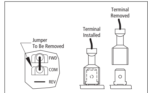
Figure 2 – Jumper Assembly
