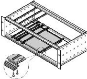
Partial width mounting plate
