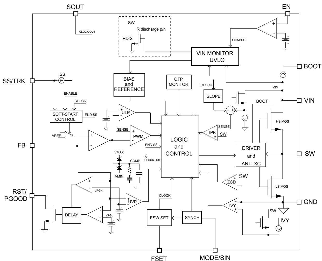
Figure 1. Block diagram
