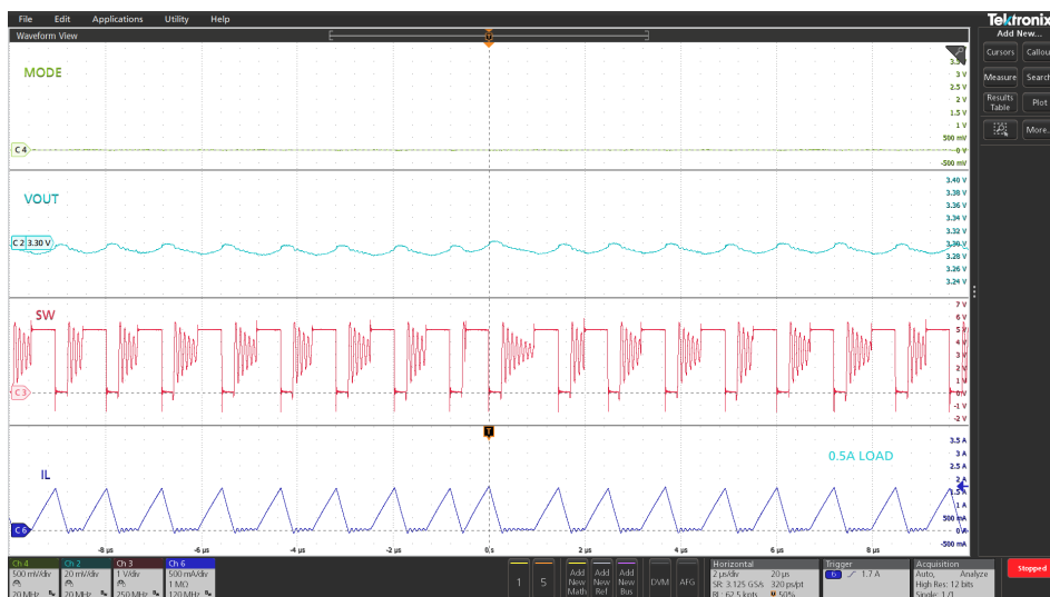
Figure 9. LCM operation, 500 mA load
