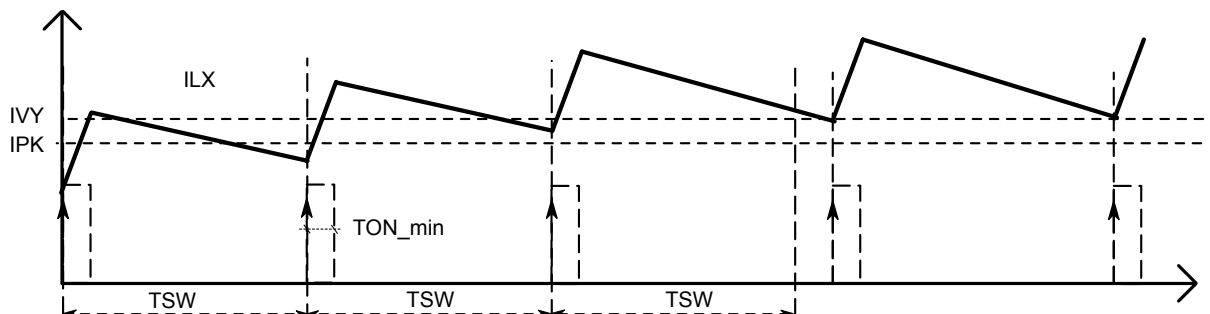
Figure 18. OCP – Valley current limit
