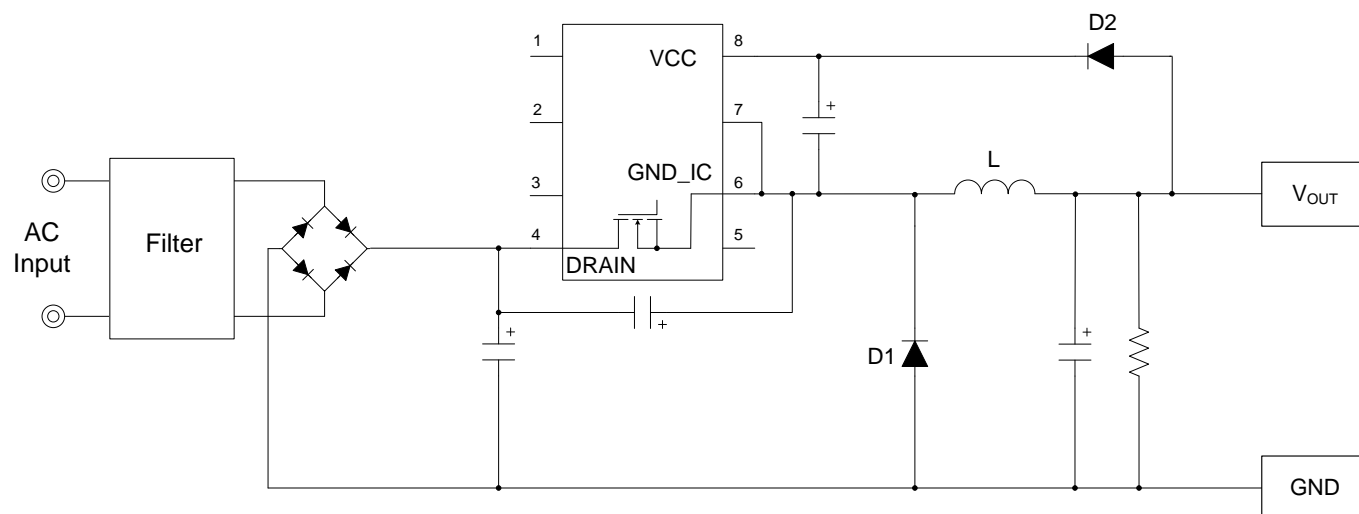
Figure 14. Application Circuit
