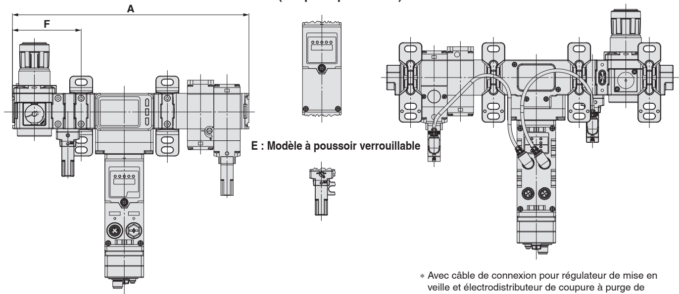
AMS20/30/40/60B-□00D (Sans raccordement)
