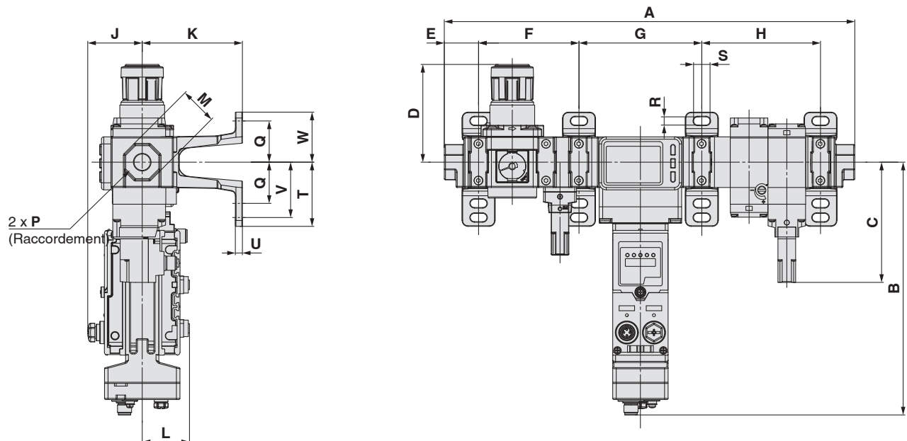
AMS20/30/40/60B-□00D (Sans raccordement)
