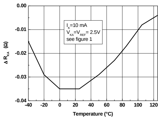
Figure 15. Drift of R_{KA} vs. temperature
