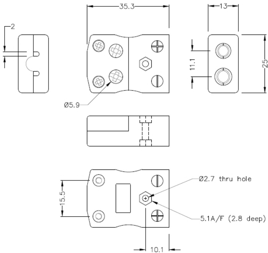
Standard in-line Socket - Quick Wire (dimensions in mm)
