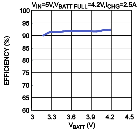
Constant Current Charge Efficiency
