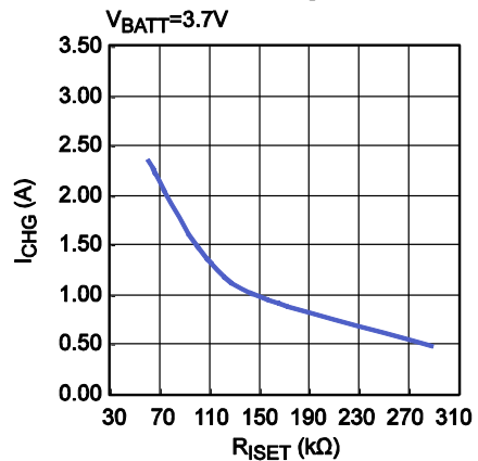
Programmable Charge Current, Charge Mode
