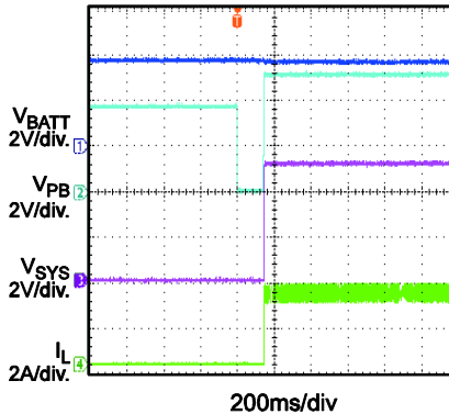
Power On by PB, Boost Mode
