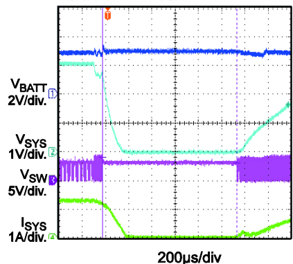
Auto Restart after SYS OCP, Boost Mode
