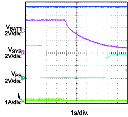
Power Off by PB, Boost Mode
