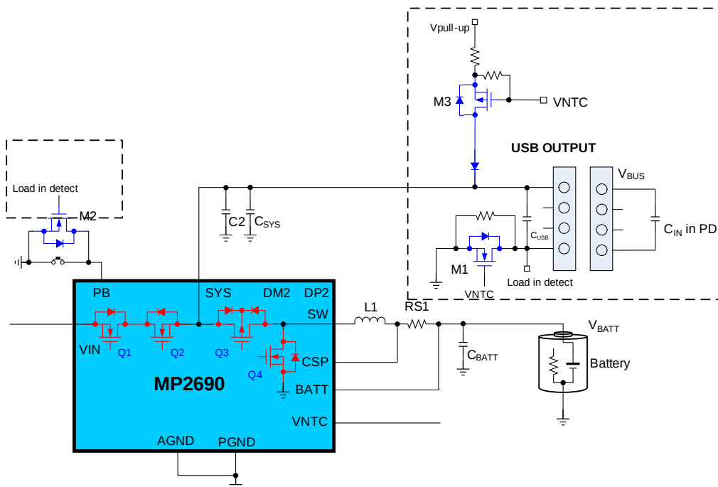
b) Low-Side MOSFET Solution
