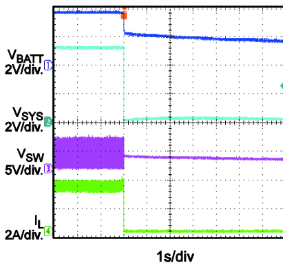
Power Off by Battery Removal, Boost Mode
