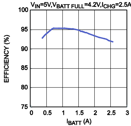
Constant Voltage Charge Efficiency
