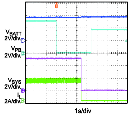
Power Off by PB, Boost Mode
