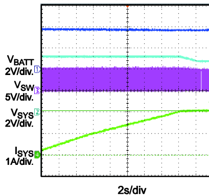
SYS Output Current Limit, Boost Mode
