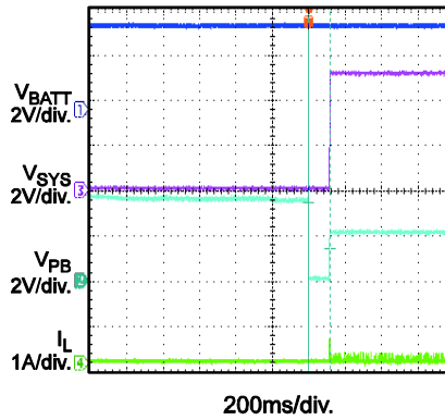
Power On by PB, Boost Mode
