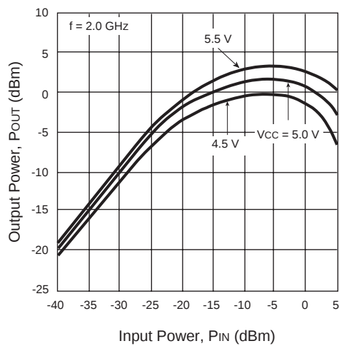
UPC2712TB OUTPUT POWER vs. INPUT POWER AND VOLTAGE
