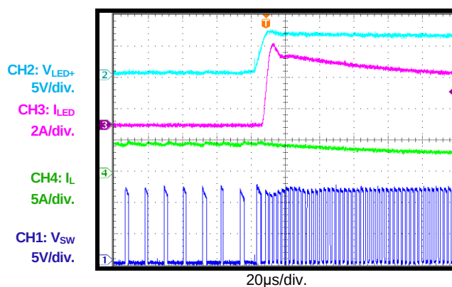
LED+ Short to VSS Recovery
