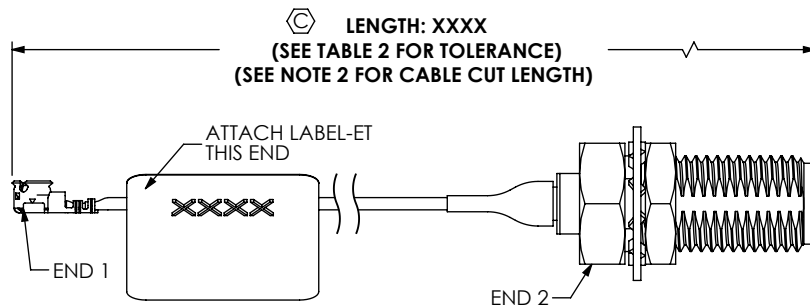
FIG 1 MHXXX-MH1RP-01BJ1-XXXX SHOWN
