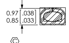
SECTION "C"- "C" SCALE 8 : 1
