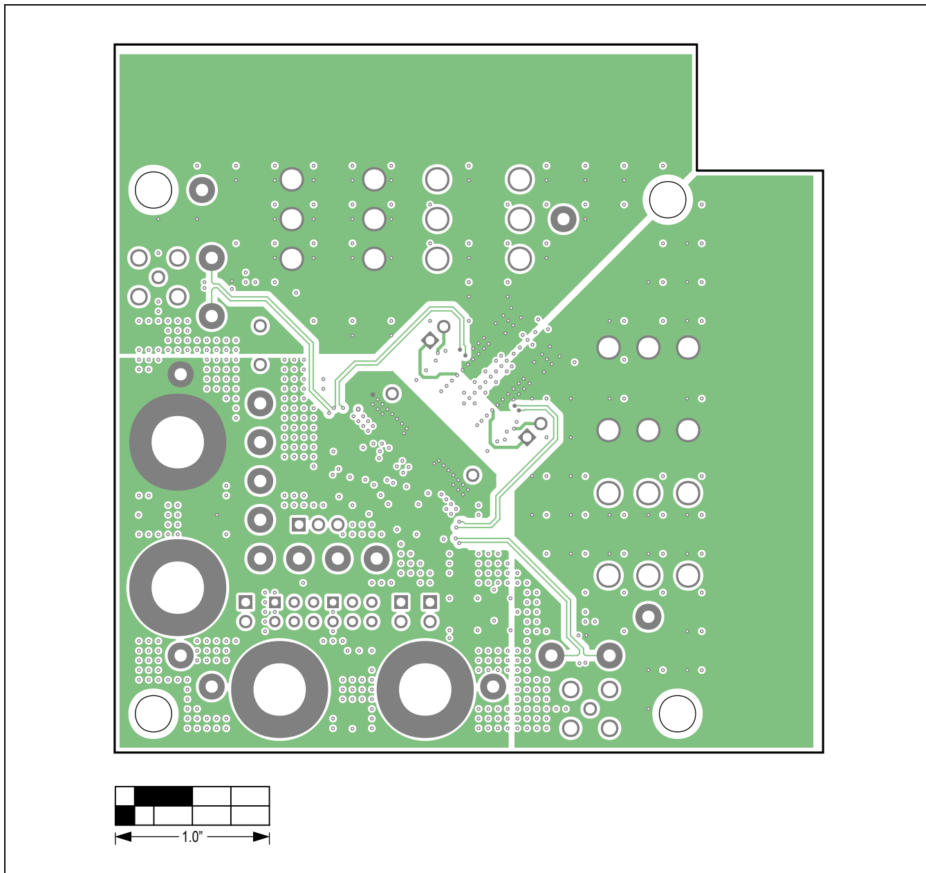
MAX20812 EV Kit PCB—Internal Layer 3
