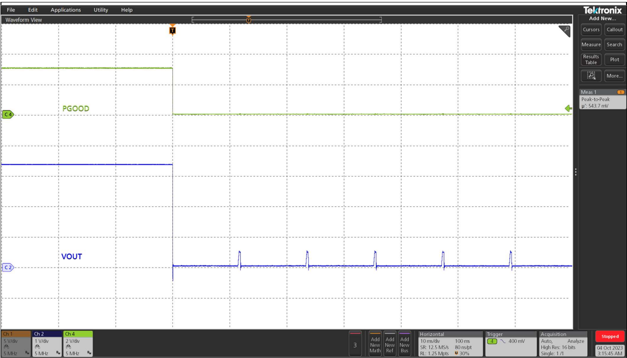
Figure 15 Short circuit and UVP (Hiccup), (Ch2: Vout, Ch4:PGood)
