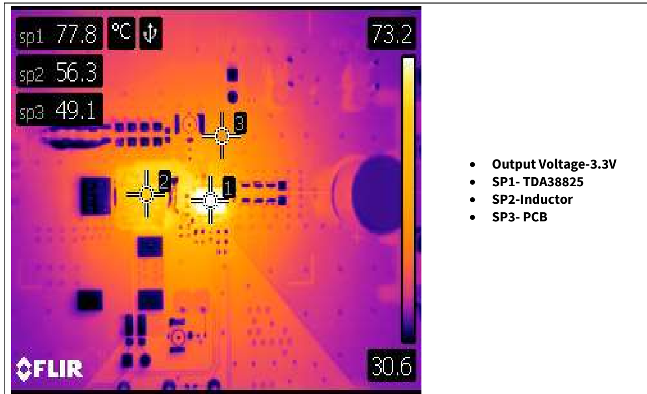
Figure 20 Thermal Performance of TDA38825 for 3.3V output voltage, 20A load, FCCM mode, 800Khz Switching Frequency, 12V Vin
