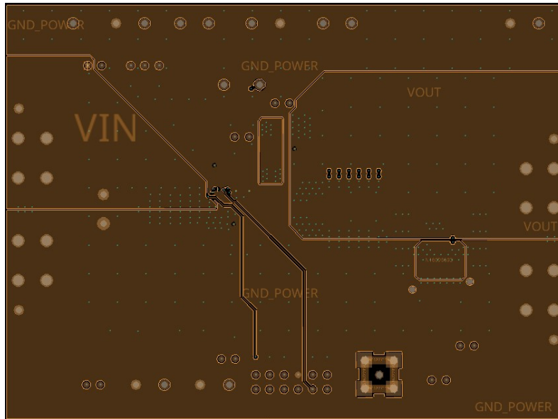
Figure 5 Inner Layer 3
