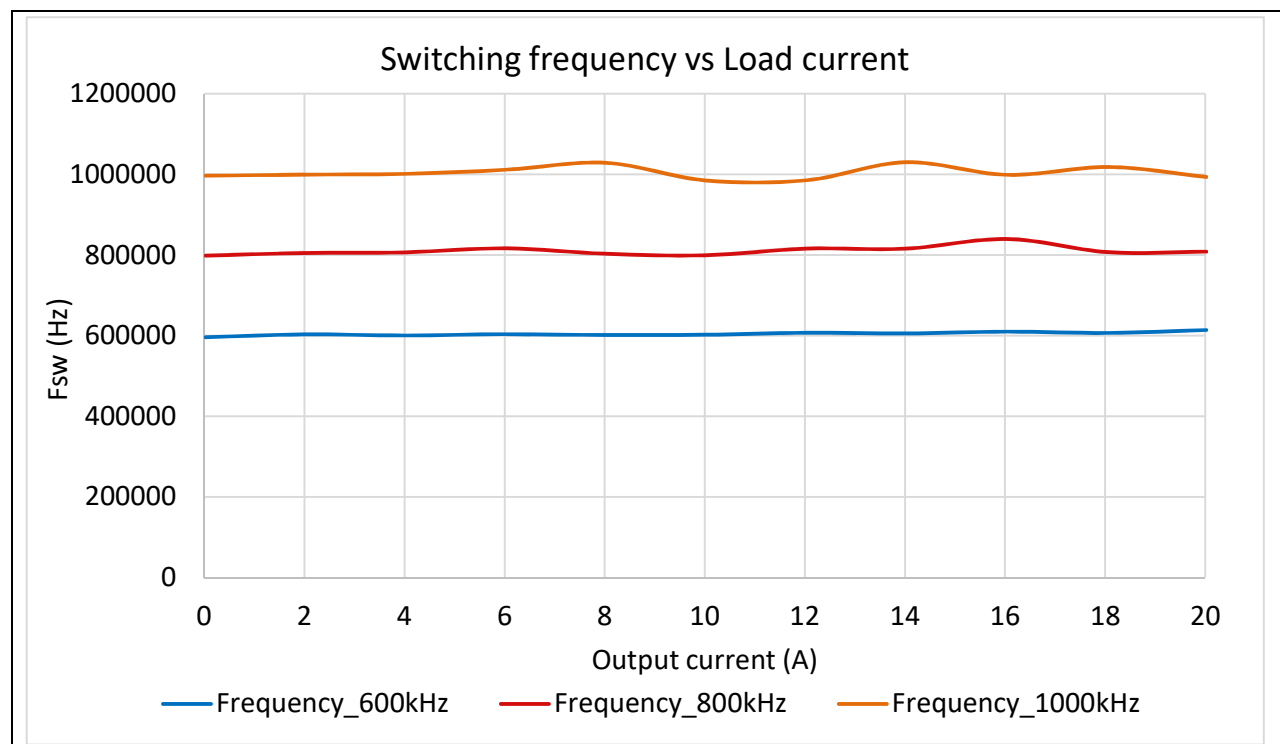
Figure 17 Switching Frequency vs Load Current
