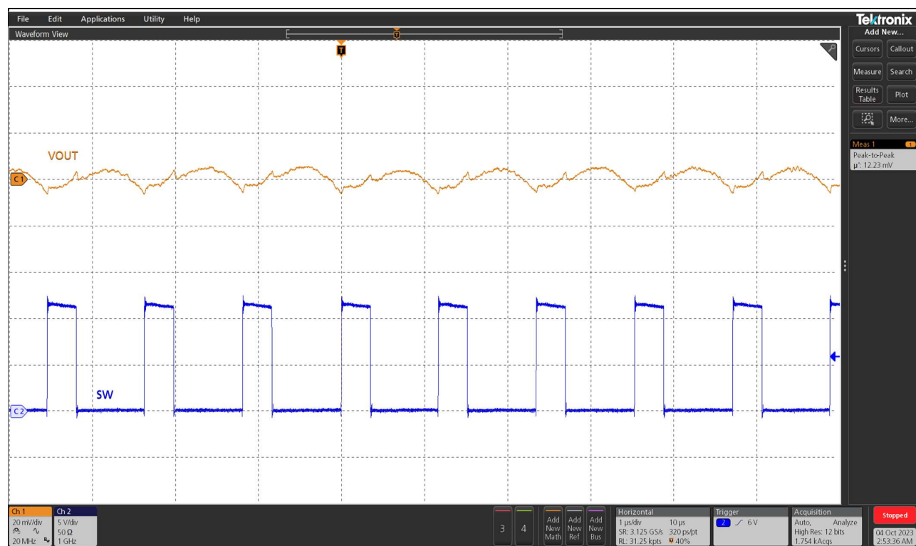
Figure 12 Vout ripple at 20A Load, fsw = 800 kHz, (Ch1: Vout, Ch2: SW)
