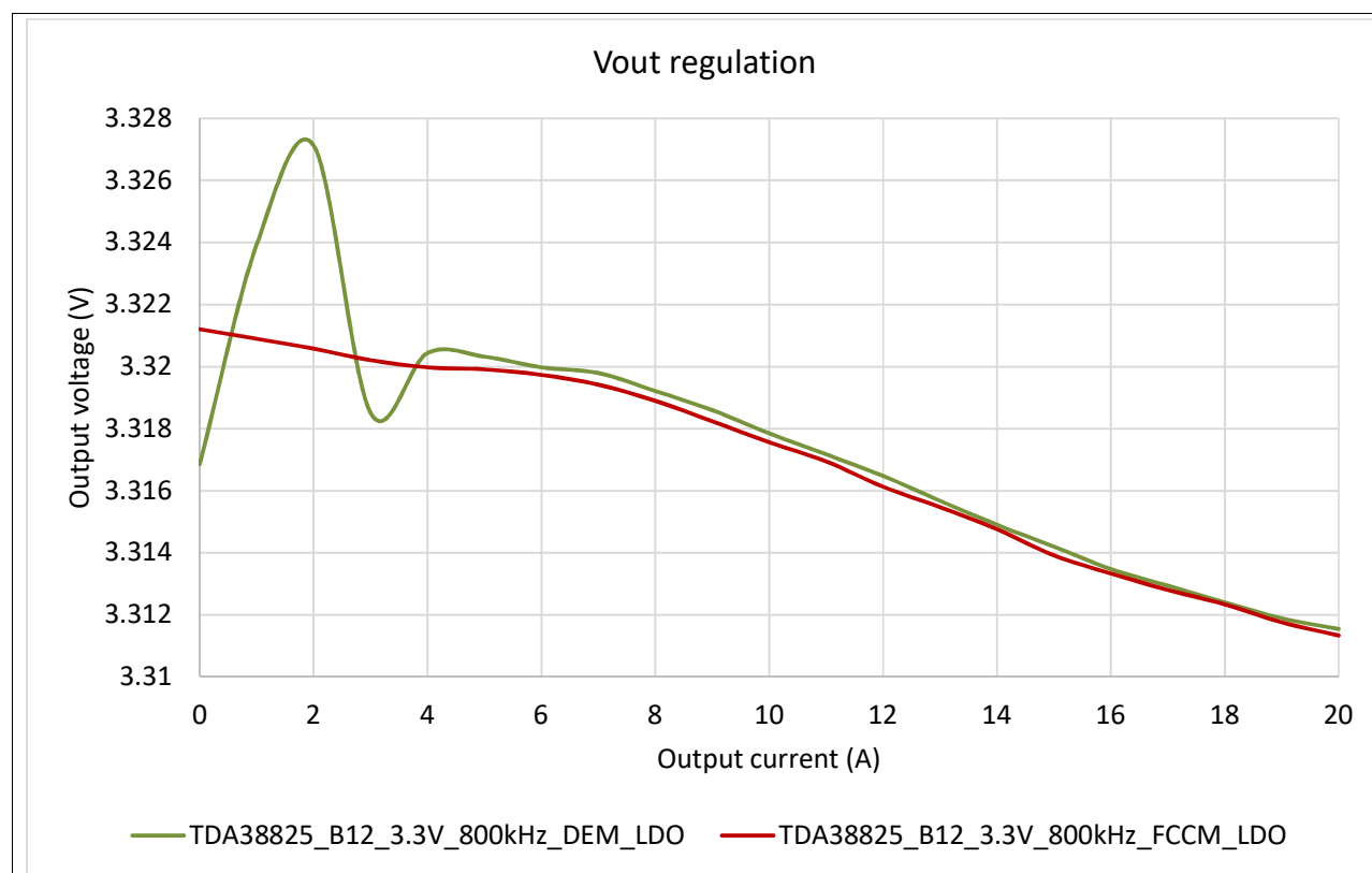
Figure 9 Output Voltage Regulation
