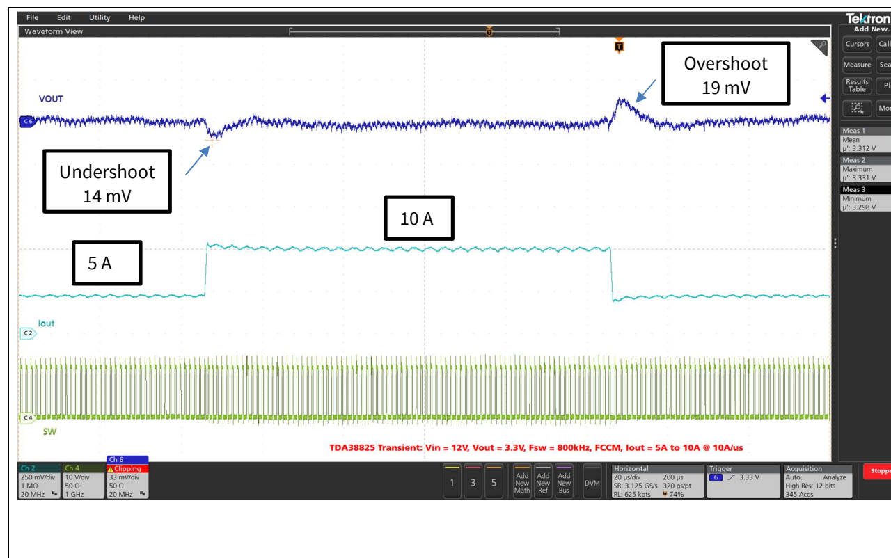
Figure 16 Transient response at 5 A step load current @ 10 A/ \mu s slew rate: I_o = 5 A – 10 A, (Ch6: V_o , Ch2: I_o , Ch4: Sw ), pk-pk: 33 mV, f_{sw} = 800 kHz
