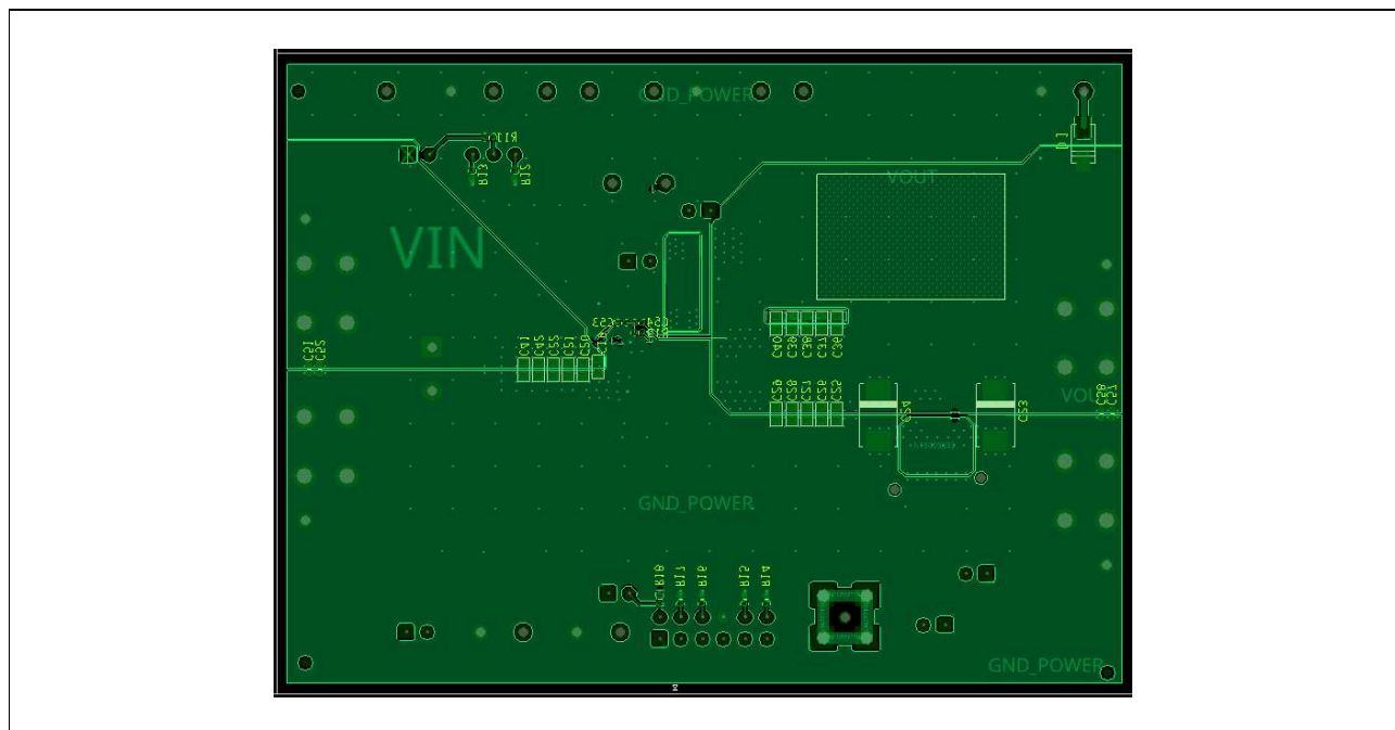
Figure 2 Bottom Layer
