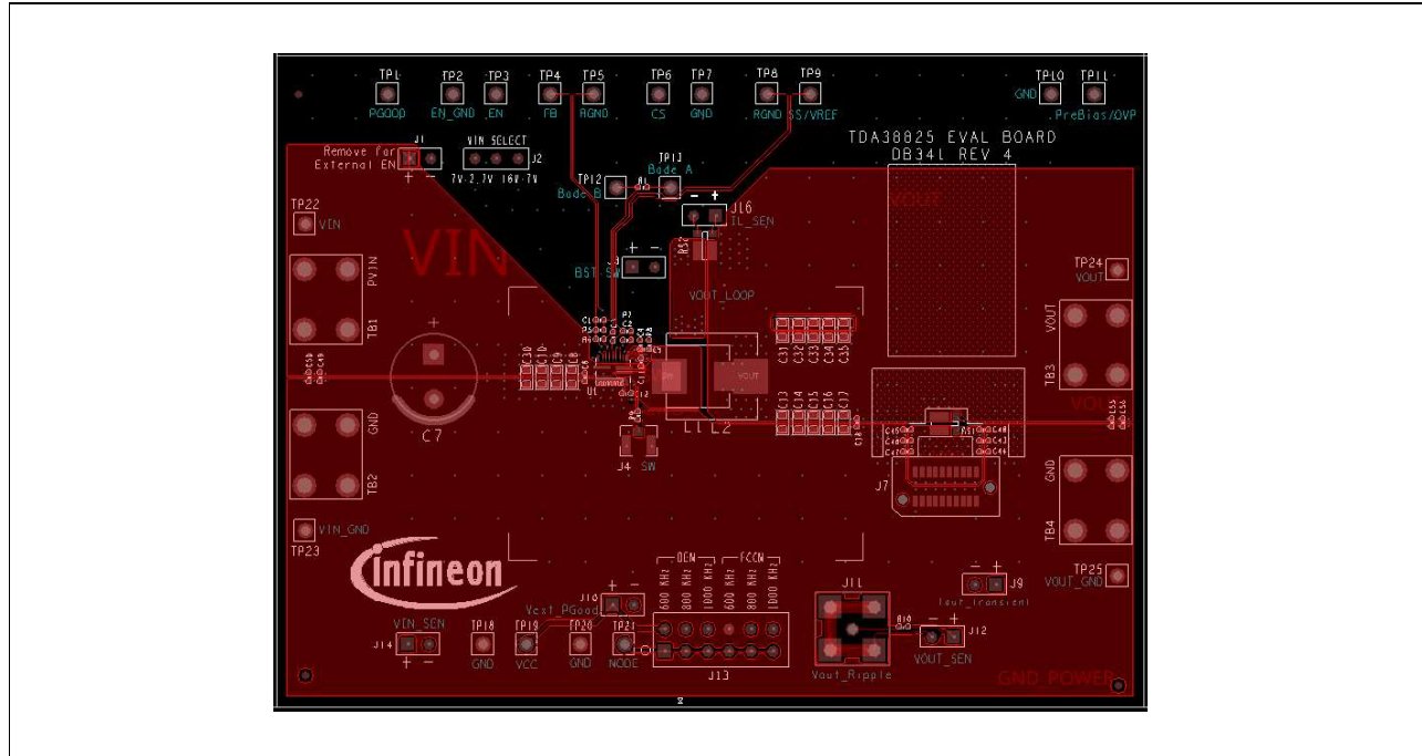
Figure 1 Top Layer
