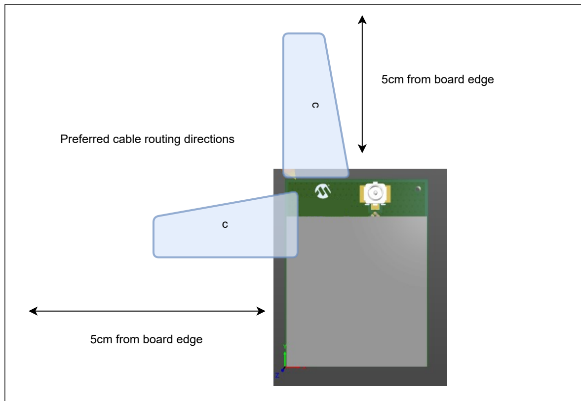
Figure 5-11. PIC32WM-BZ6204 Antenna Placement Guidelines
