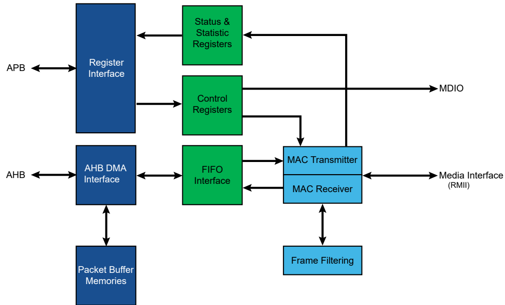
Figure 45-1. Block Diagram
