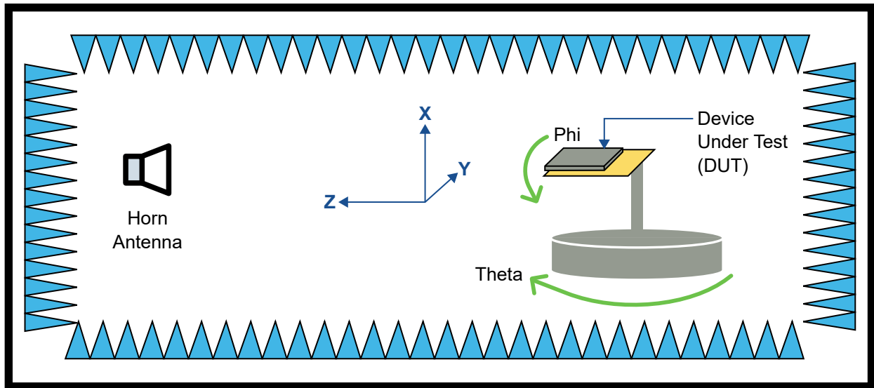
Figure 5-12. Chip Antenna Radiation Pattern Placement
