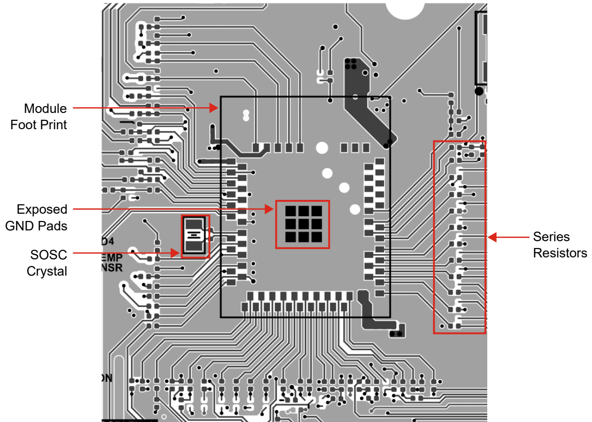
Figure 5-9. Example of Host Board on Top Layer – PIC32WM-BZ6204 Module
