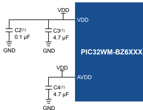
Figure 5-5. Recommended Module Power Supply Connections
