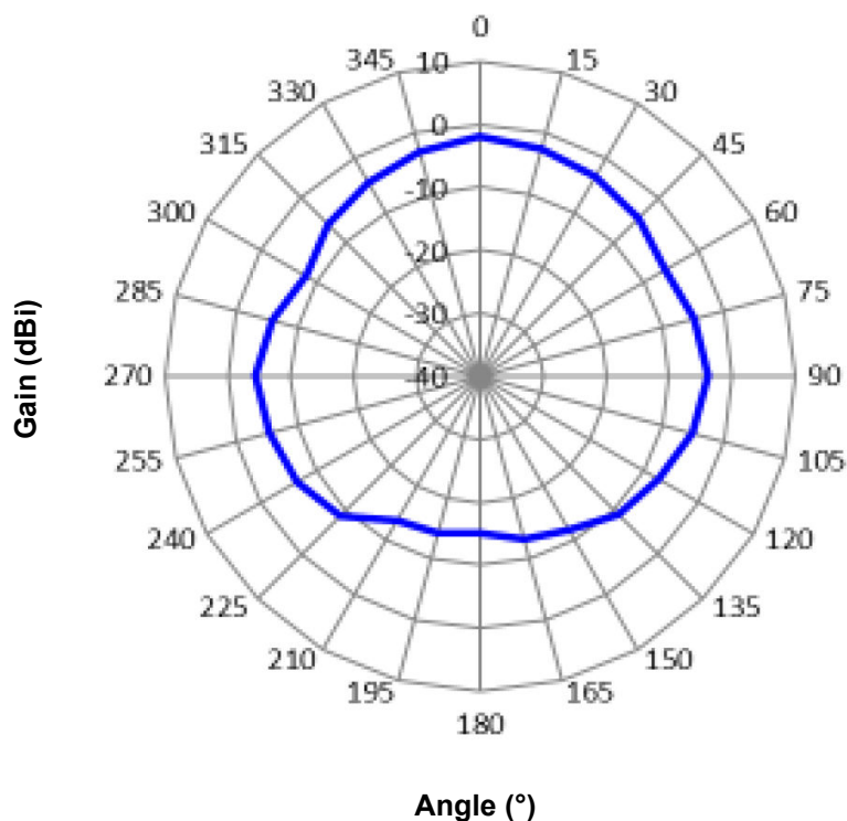
Figure 5-15. PIC32WM-BZ6602 Antenna Radiation Pattern when \Theta = 90^\circ
