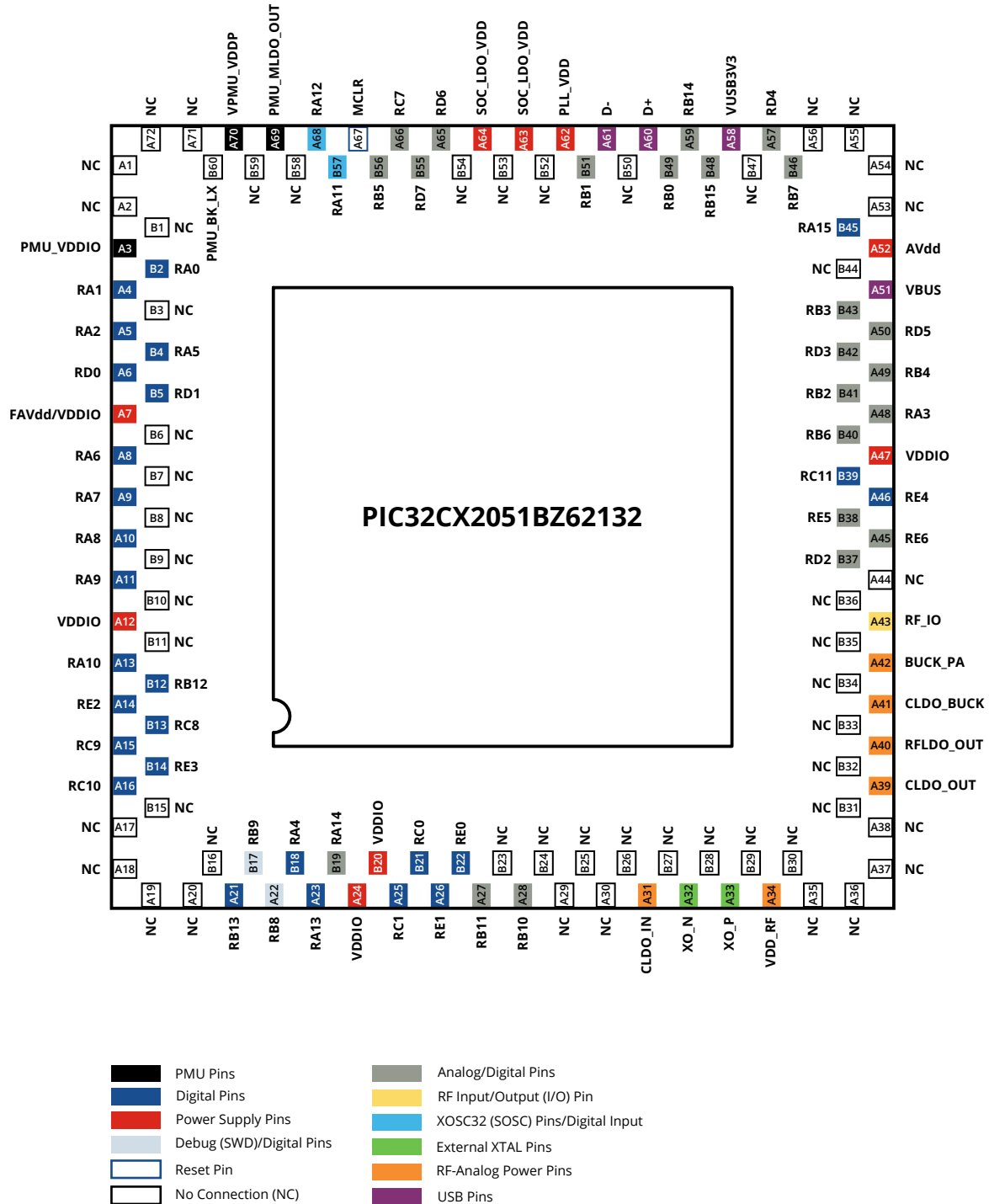
Figure 4-3. PIC32CX2051BZ62132 Pinout Diagram – Top View
