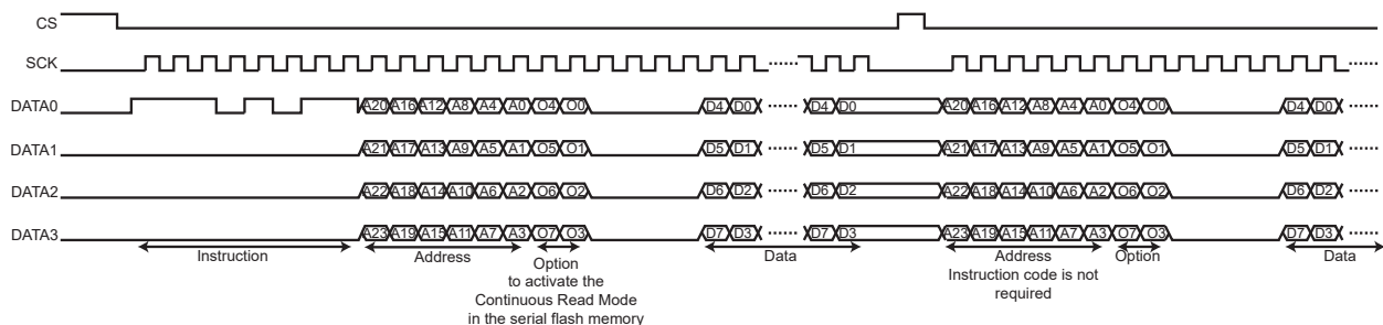
Figure 36-11. Continuous Read Mode
