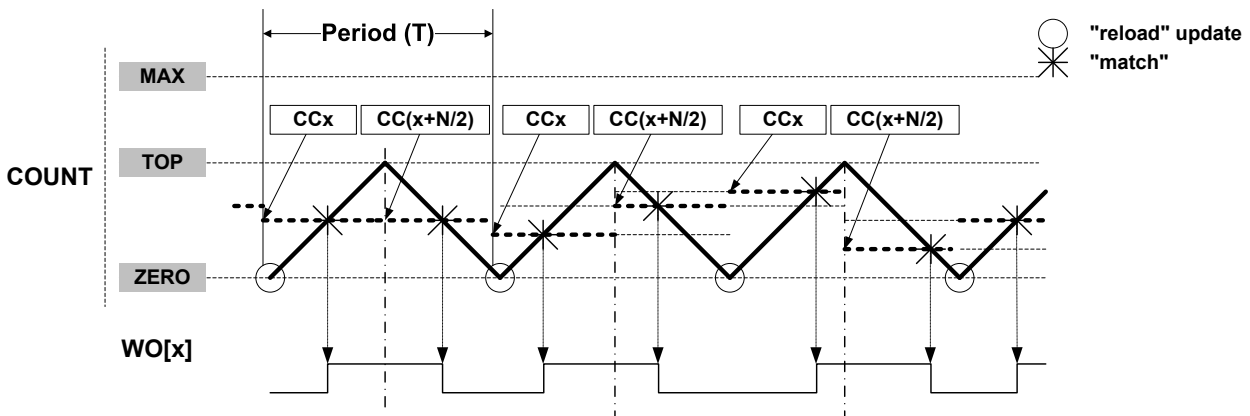
Figure 42-8. Dual-Slope Critical Pulse Width Modulation ( N=\text{CC\_NUM} )
