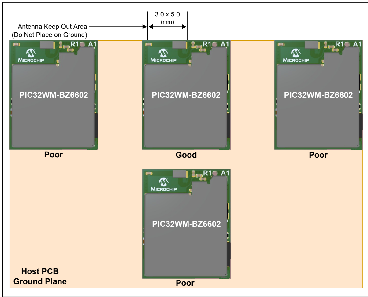
Figure 5-8. PIC32WM-BZ6602 Module Placement on Host Board
