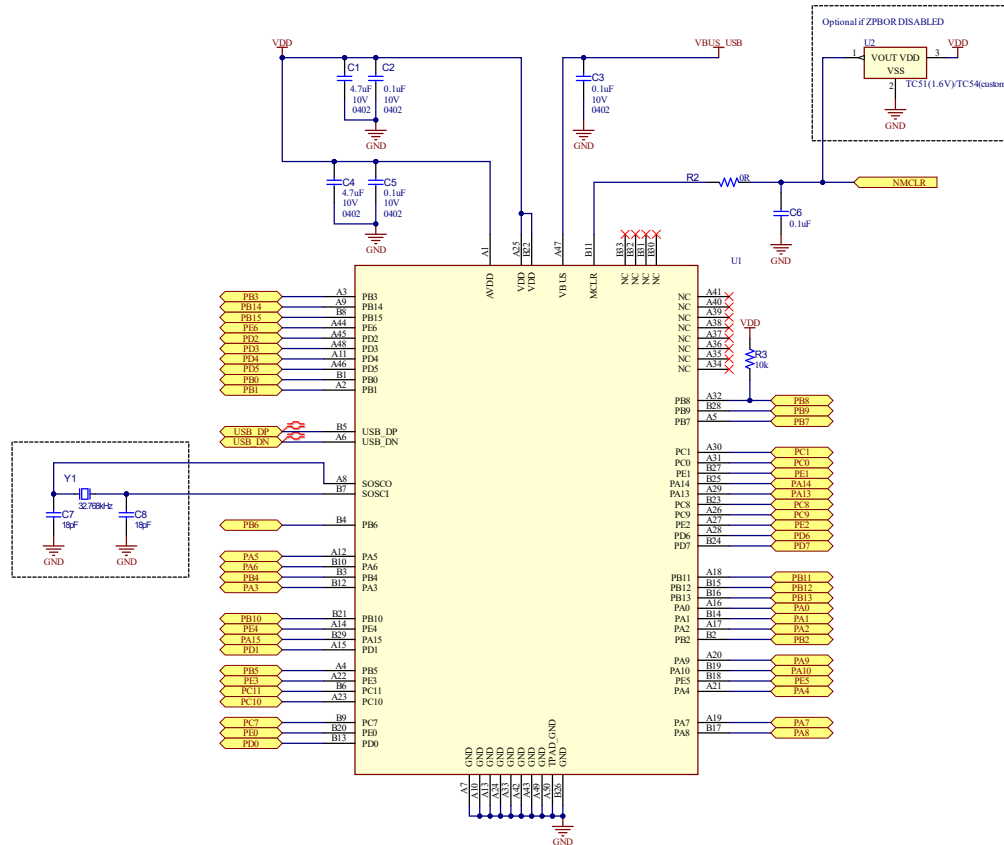
Figure 5-4. Module Basic Connection and Interface Diagram for PIC32WM-BZ6602 Module
