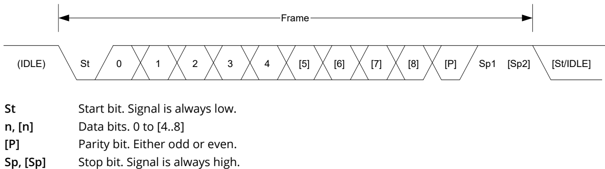
Figure 33-2. Frame Formats
