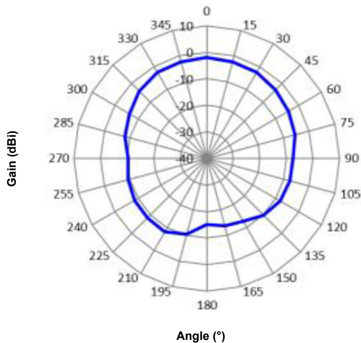
Figure 5-13. PIC32WM-BZ6602 Antenna Radiation Pattern when \Phi = 0^\circ
