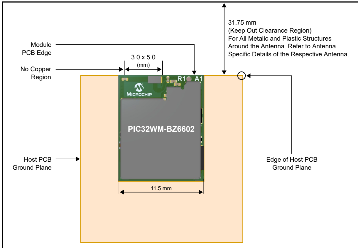
Figure 5-7. PIC32WM-BZ6602 Module Placement Guidelines
