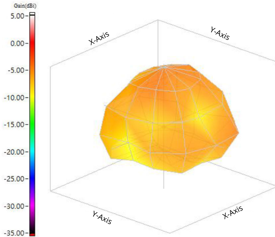
Figure 5-16. PIC32WM-BZ6602 Antenna Radiation 3D Pattern
