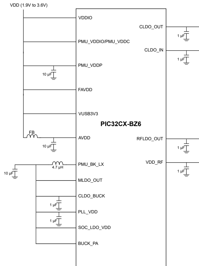
Figure 8-2. Typical Power Supply Connection for SoC
