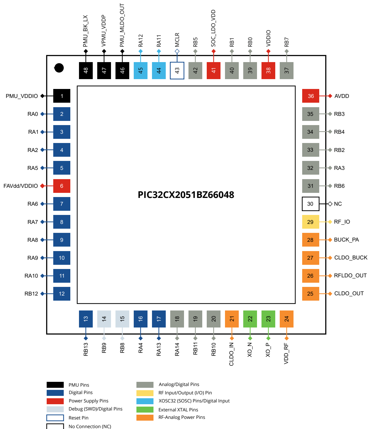
Figure 4-4. PIC32CX2051BZ66048 Pinout Diagram – Top View
