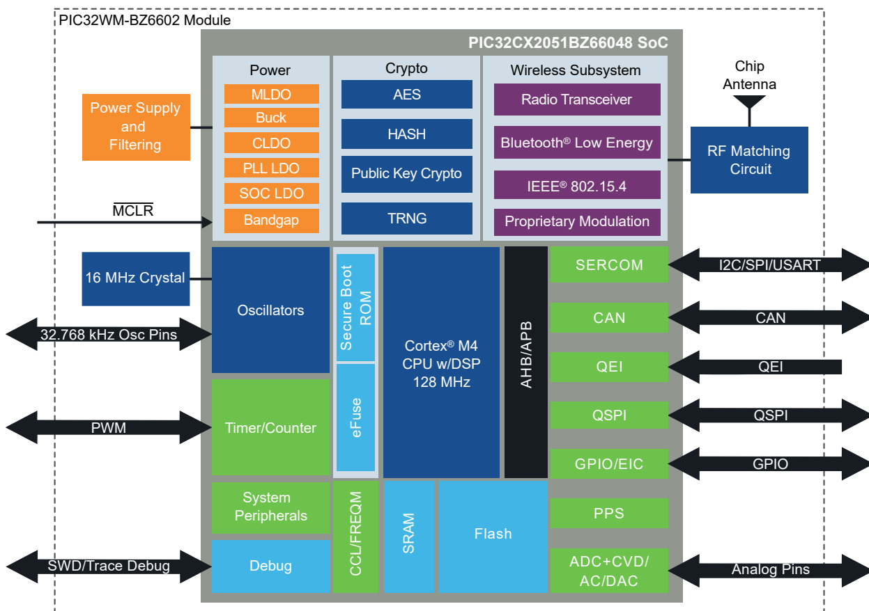
Figure 5-2. PIC32WM-BZ6602 Module Block Diagram
