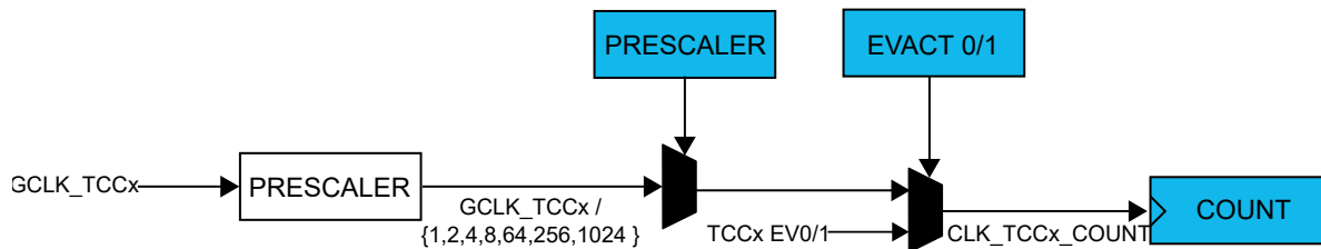
Figure 42-2. Prescaler
