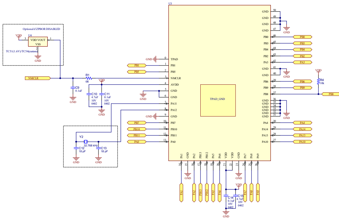
Figure 5-4. Module Basic Connection and Interface Diagram for PIC32WM-BZ6602 Module
