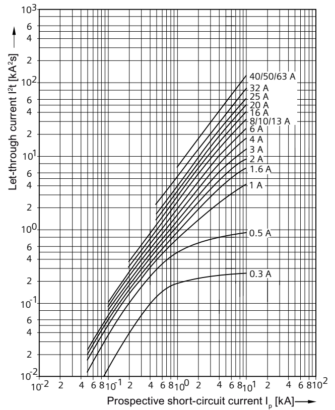
Characteristic D
