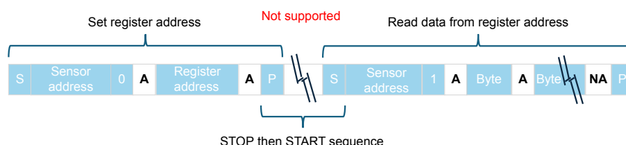
Figure 25. Incompatible I 2 C read sequence
