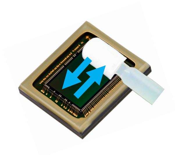
Figure 33. Step two
