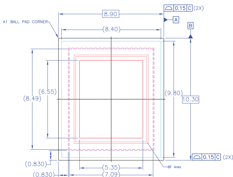
Figure 29. Top view
