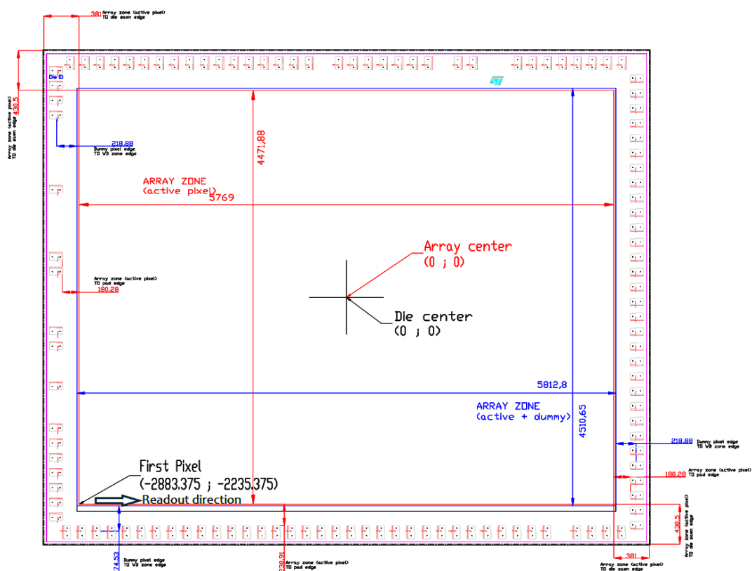
Figure 34. Die pad positions (see-through view)
