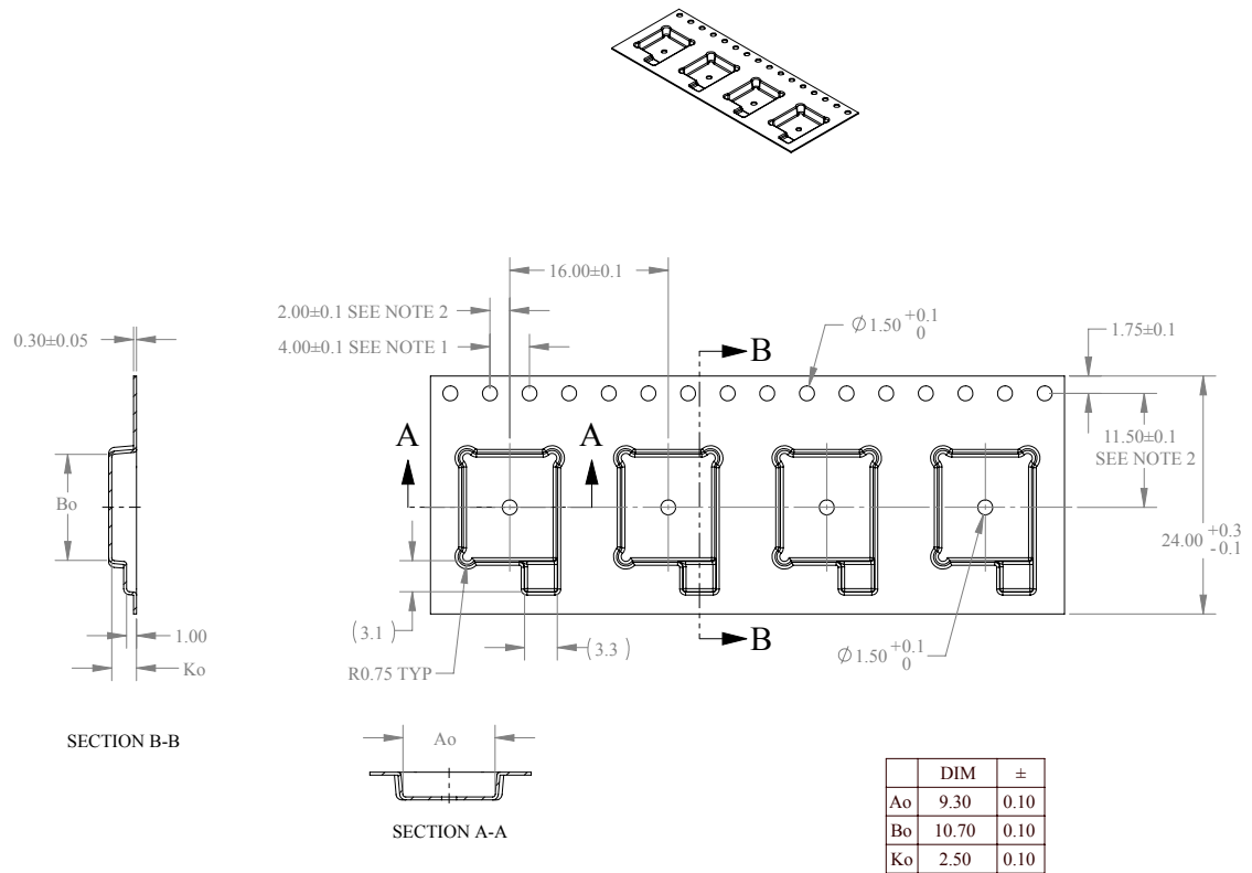
Figure 38. Carrier tape
