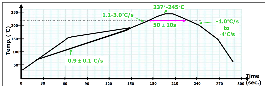
Figure 40. Soldering temperature vs time
