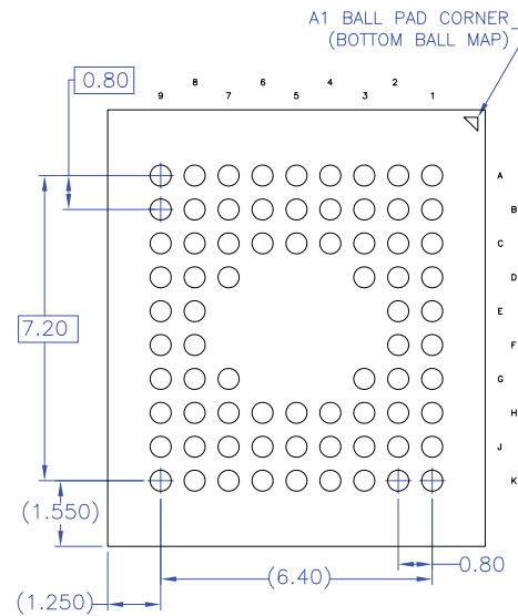
Figure 30. Bottom view
