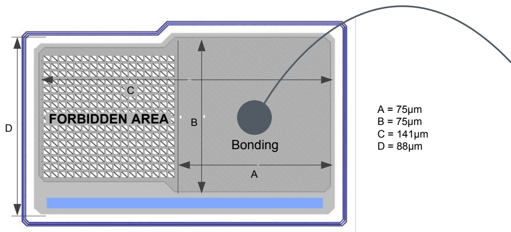
Figure 36. Bonding pad opening
