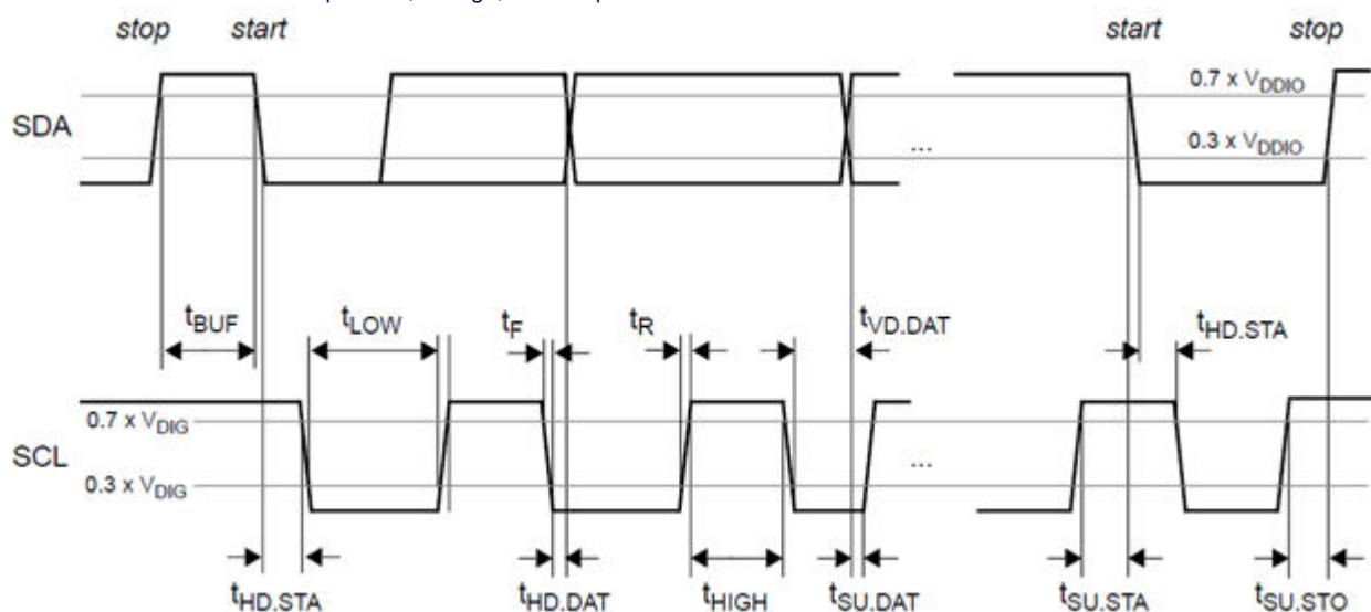
Figure 41. I 2 C timing
