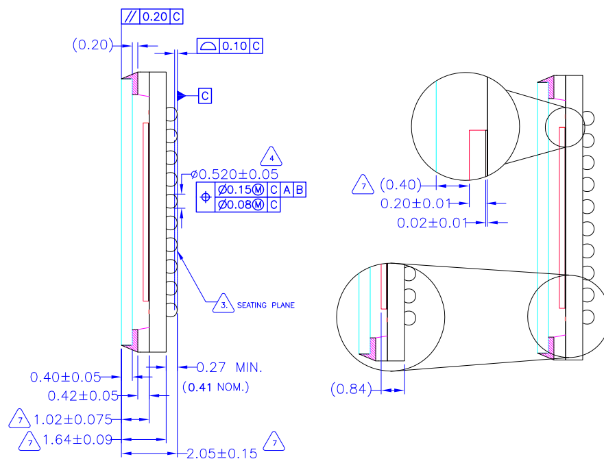
Figure 31. Side view
