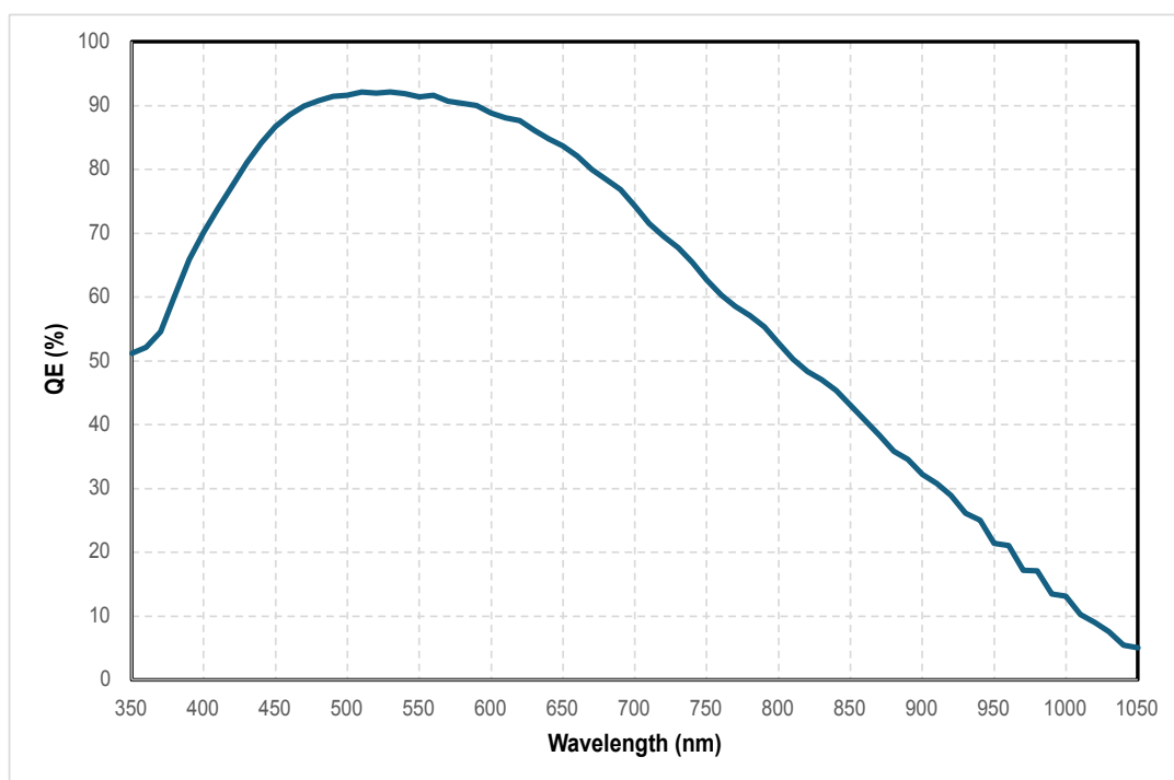
Figure 3. QE (60°C)
