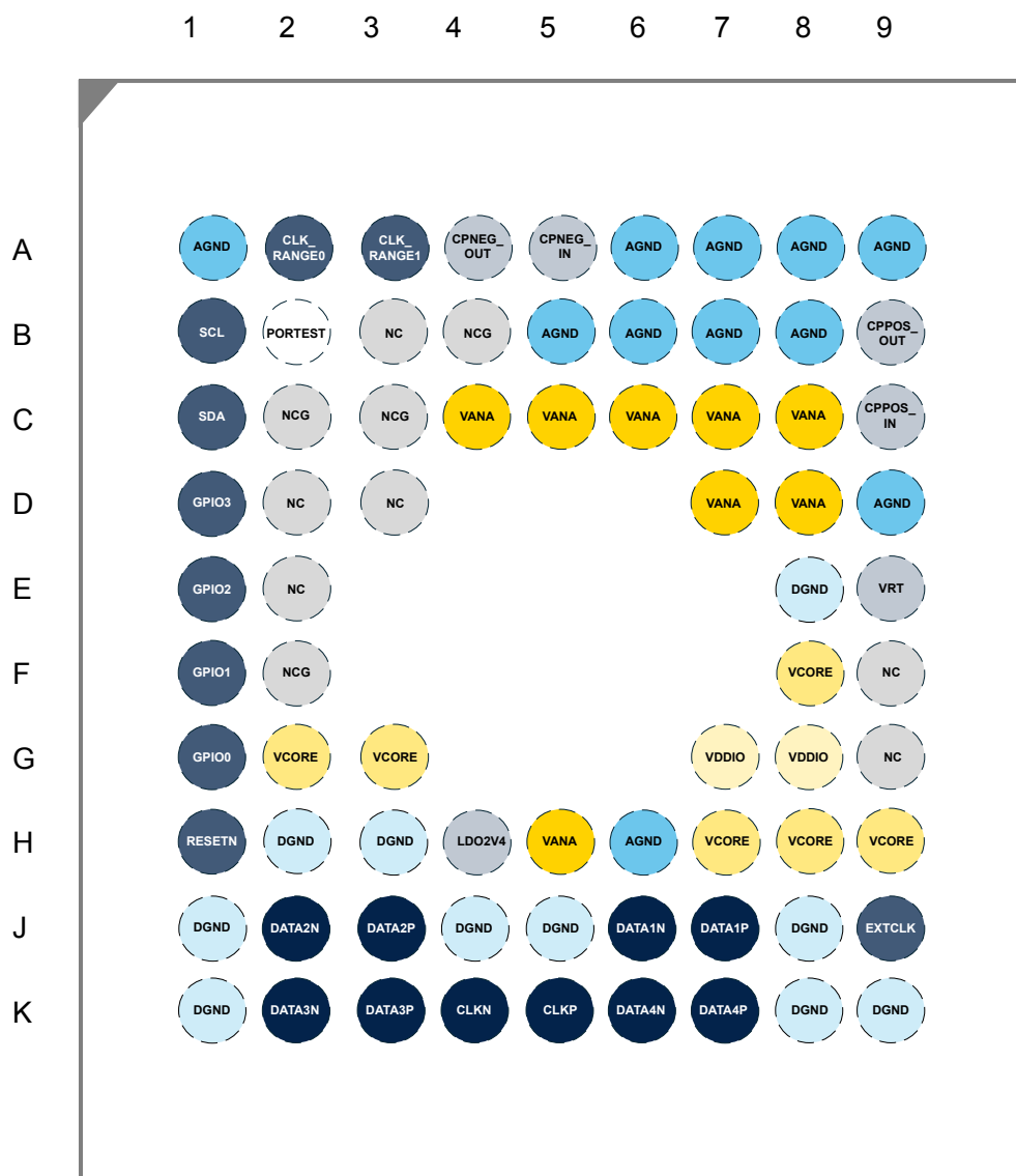
Figure 7. Ball assignment (see-through view)
