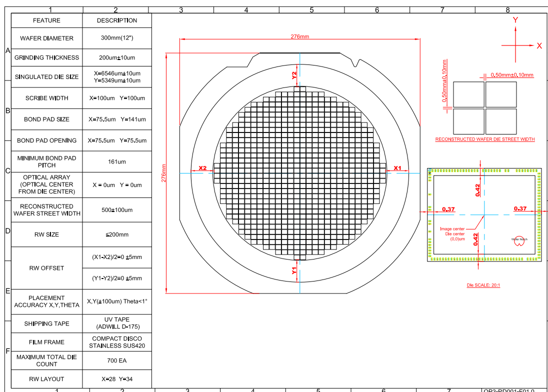
Figure 39. Reconstructed wafer information
