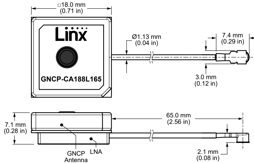
Figure 6. ANT-GNCP-CA188L165 Antenna Dimensions
