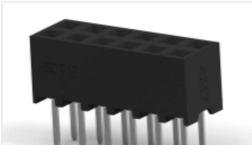
TE Part #1-2314822-2 12P,2MM,B-B,REC,DRVT,2.7,0.76AU,TB
