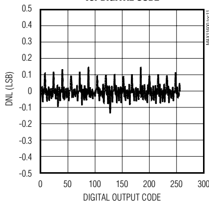
DIFFERENTIAL NONLINEARITY vs. DIGITAL CODE
