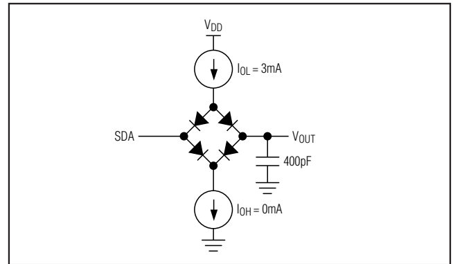
Figure 2. Load Circuit
