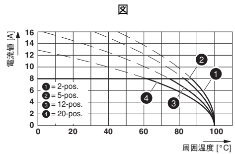
Type: FMC 1,5/...-ST-3,81 with MCV 1,5/...-G-3,81 P.. THR
