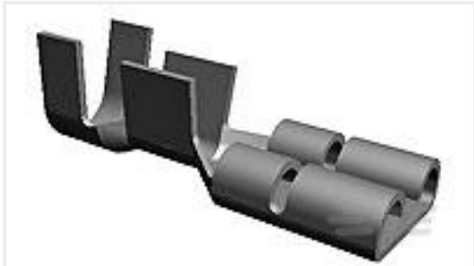
TE Part #444335-2 250 FASTON REC 16-14 AWG TPBR
