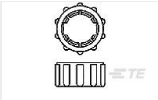
TE Part #213810-1 CPC COUPLING RING SIZE 17
