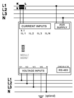
3P4W BALANCED
