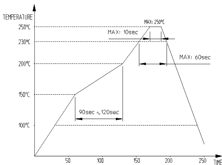
[Fig.1] REFLOW TEMPERATURE
