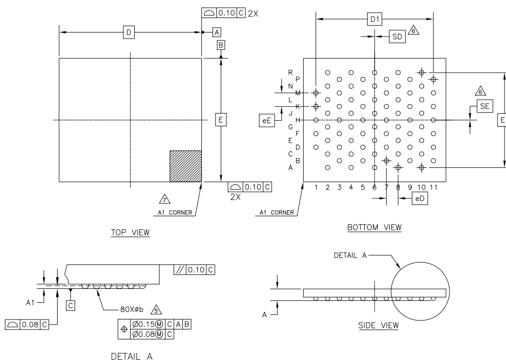
Figure 6. Thin 80-Ball WLCSP 3.676 × 3.190 × 0.33 mm
