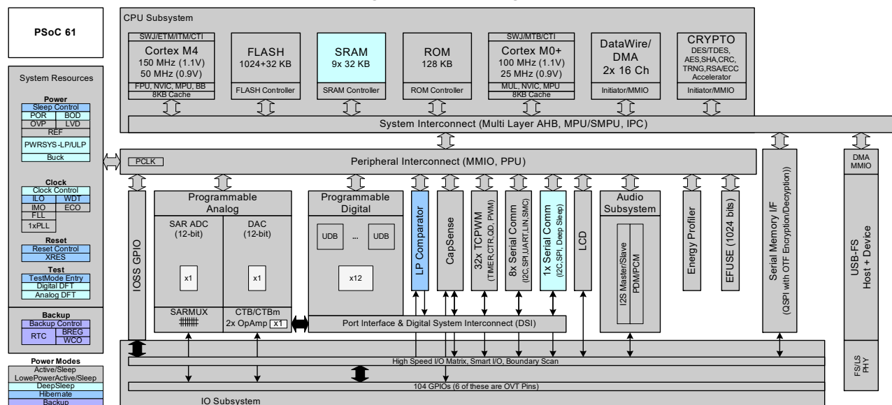
Figure 2. Block Diagram
