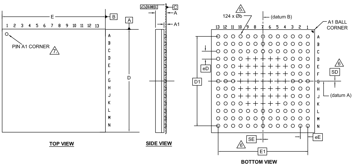
Figure 4. 124-BGA 9.0 × 9.0 × 1.0 mm
