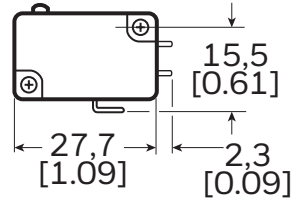
Figure 7. Short Solder
