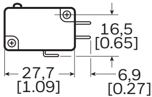
Figure 6. Solder
