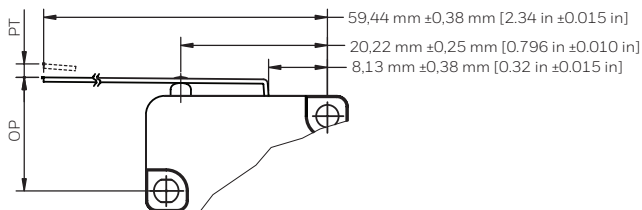
Figure 10. Long Straight Lever
