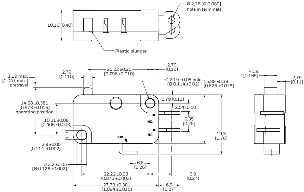
Figure 1. V3 Series Standard Switch Dimensions
