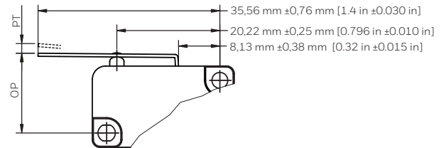
Figure 9. Standard Straight Lever
