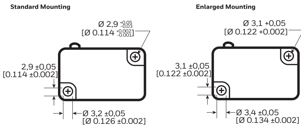
Figure 2. V3 Series Mounting Dimensions
