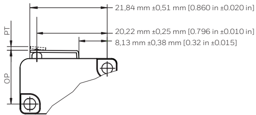
Figure 8. Straight Short Lever
