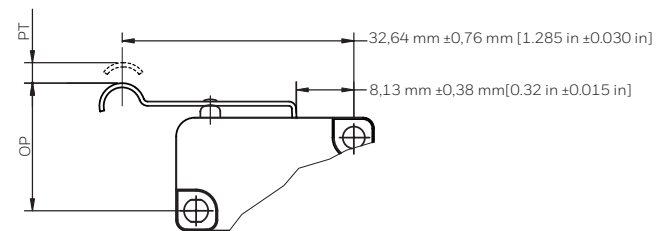
Figure 11. Simulated Roller Lever
