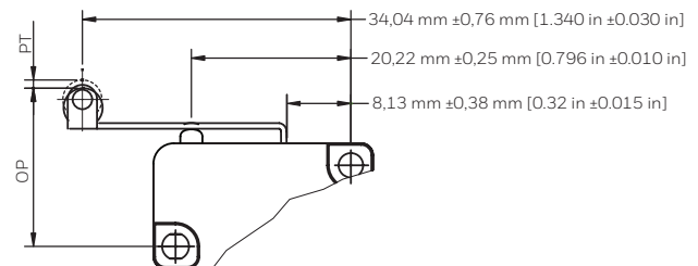
Figure 13. Roller Lever
