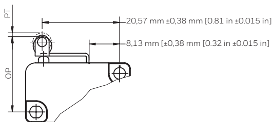
Figure 12. Short Roller Lever
