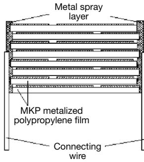
MKP385 (1600 V to 2000 V) Extended metalized film with internal series connections (3 sections) design
