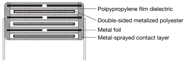
KP1836 Extended foil design with internal series connection and double-sided metalized carrier film
