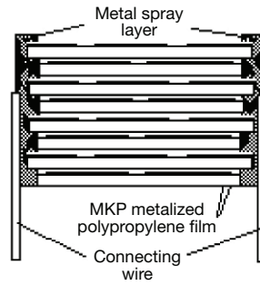
MKP385 (2500 V) Extended metalized film with internal series connections (4 sections) design
