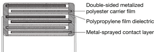
MMKP383 (250 V to 630 V) Extended double-sided metalized film design
