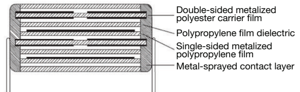
MMKP383 (1000 V to 1400 V) Extended double-sided metalized film with internal series connection design
