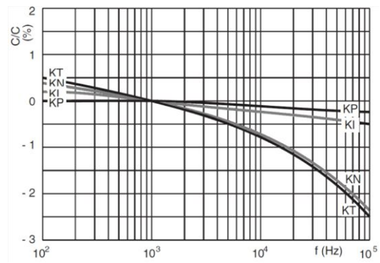
Capacitance change as a function of frequency at room temperature (typical curve)
