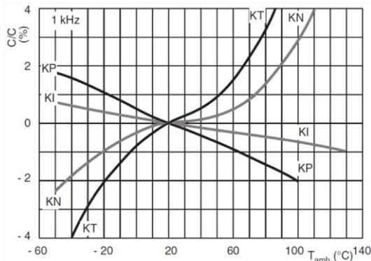
Capacitance change at 1 kHz as function of temperature (typical curve)
