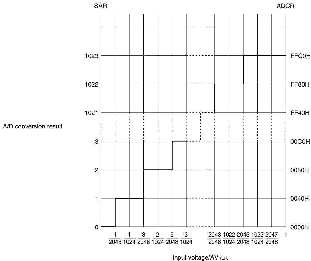
Figure 11-13. Relationship Between Analog Input Voltage and A/D Conversion Result
