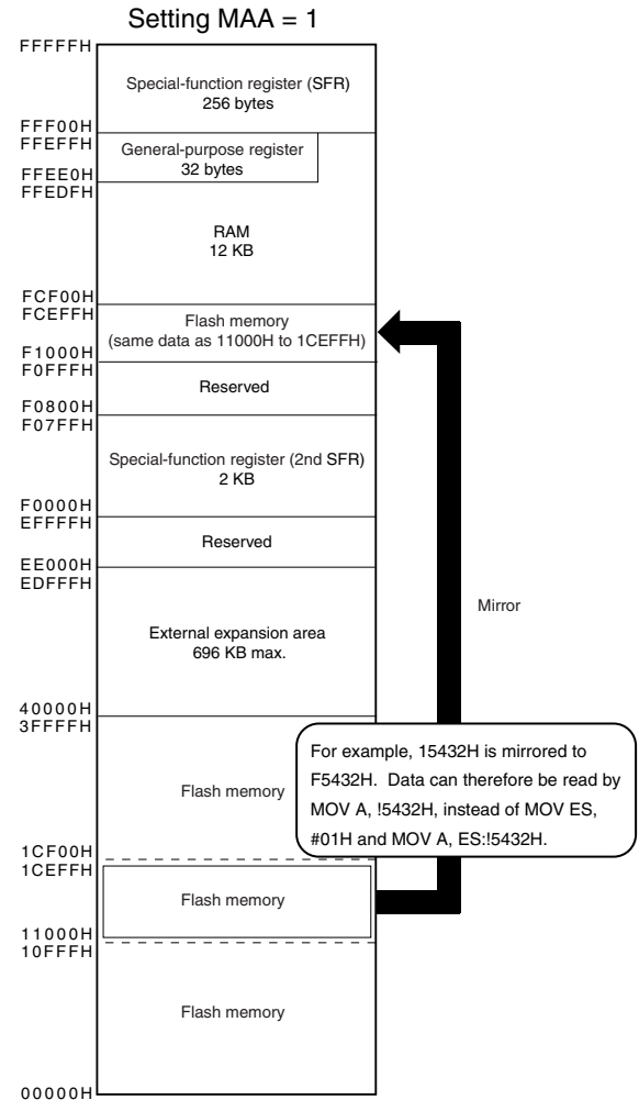
Example 2 \mu PD78F1166, 78F1166A (Flash memory: 256 KB, RAM: 12 KB)
