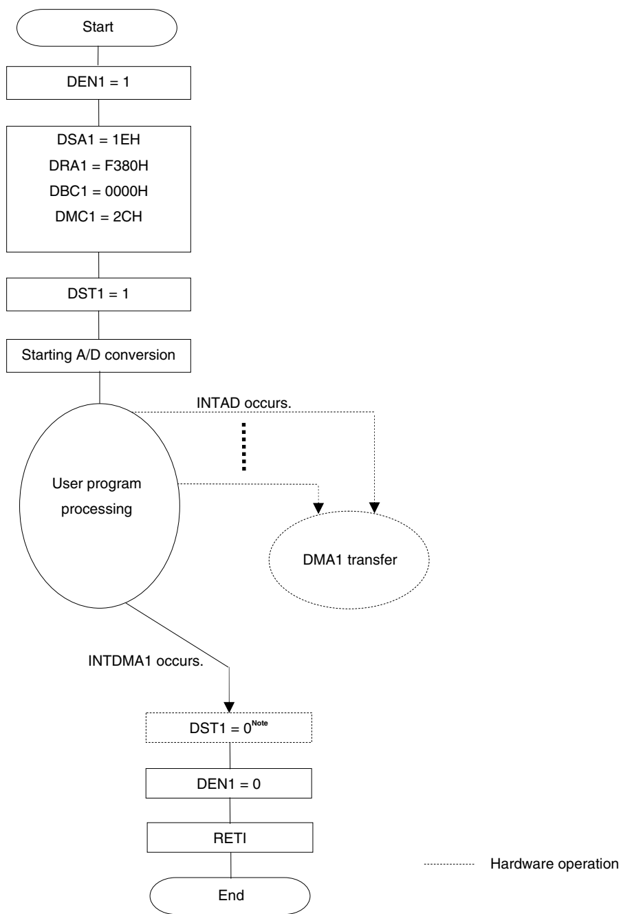
Figure 16-10. Setting Example of Consecutively Capturing A/D Conversion Results
