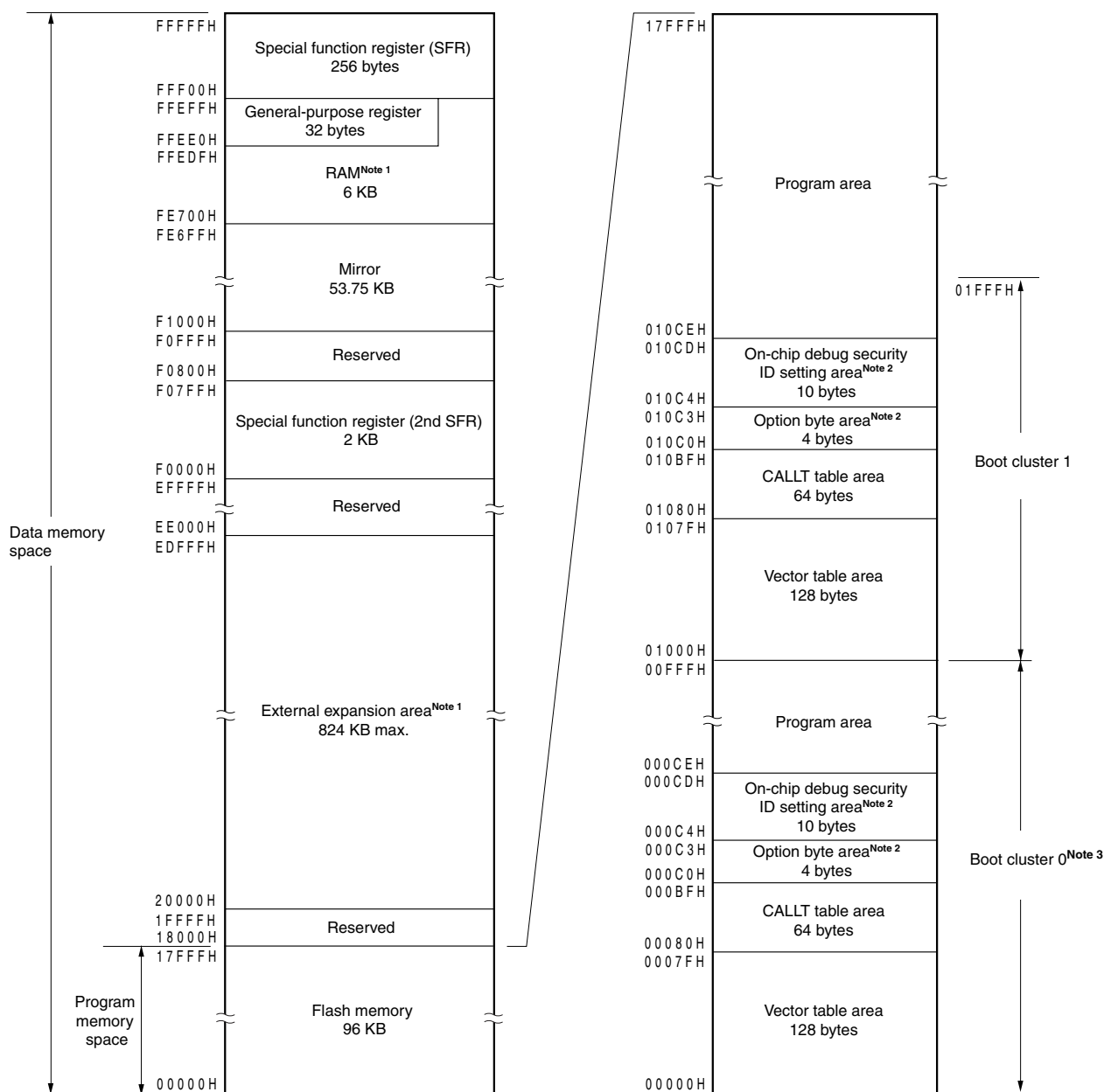
Figure 3-2. Memory Map (μPD78F1163, 78F1163A)
