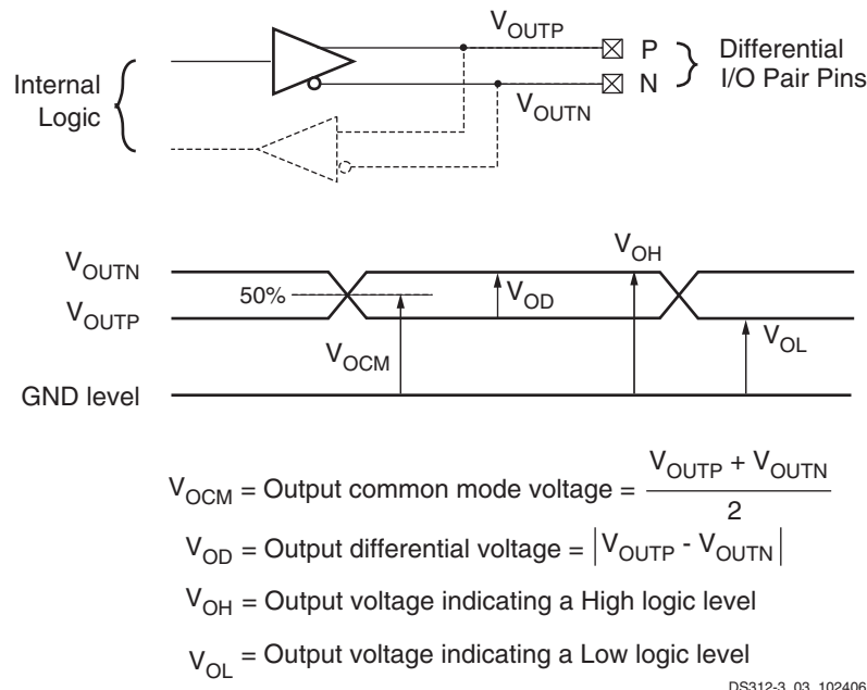
Figure 4: Differential Output Voltages
